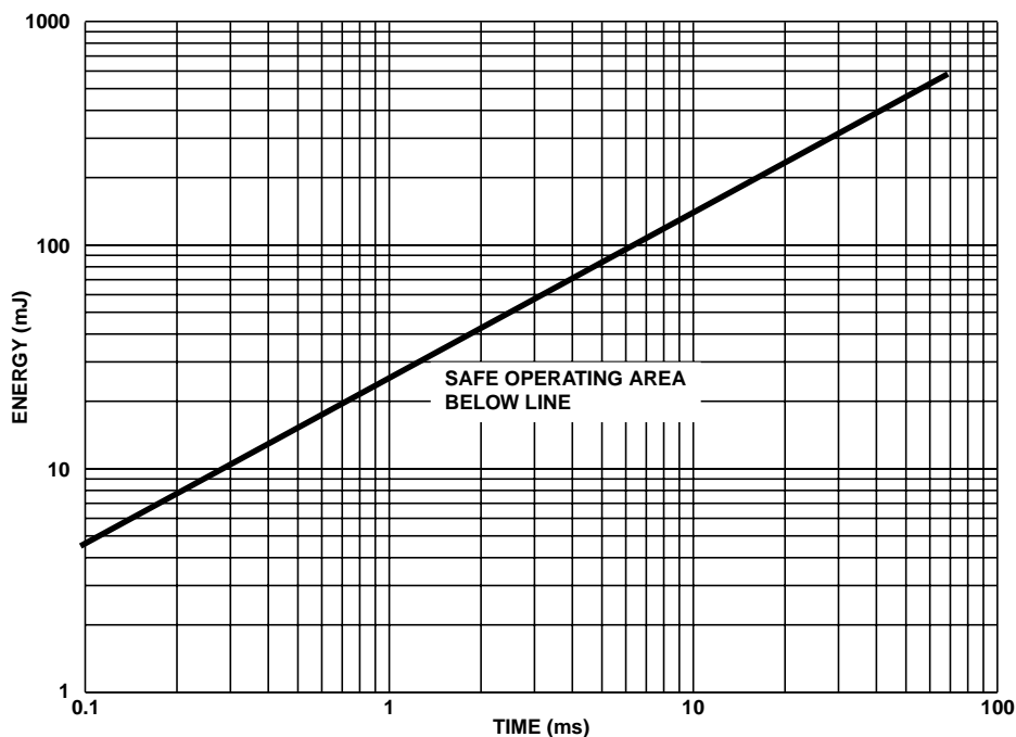
FIGURE 2. MAXIMUM SINGLE PULSE ENERGY SAFE OPERATING AREA FOR EACH CLAMPED OUTPUT DRIVER, T_A = 25^\circ\text{C}
