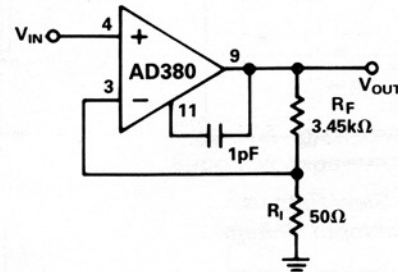
Figure 30. Video Amplifier
