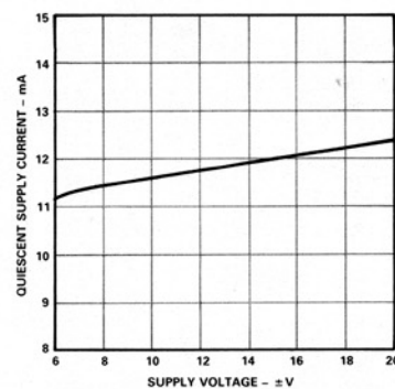
Figure 11. Supply Current vs. Supply Voltage
