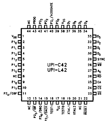
290414-3 Figure 3. QFP Pin Configuration
