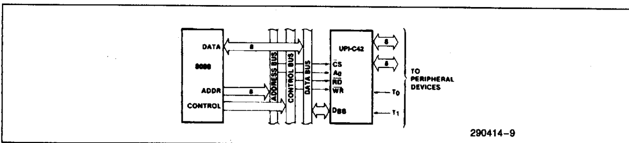
Figure 8. 8088-UPI-C42 Interface
