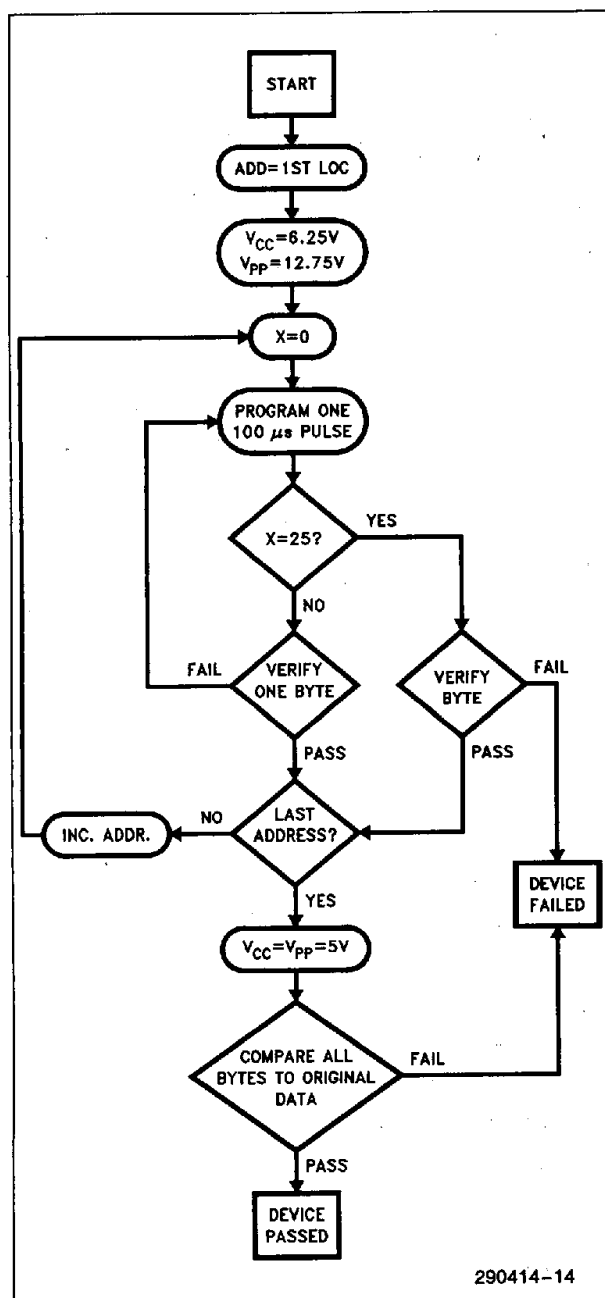
Figure 6. Quick-Pulse Programming Algorithm
