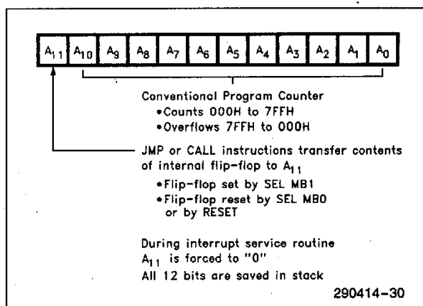
Figure 5. Program Counter
