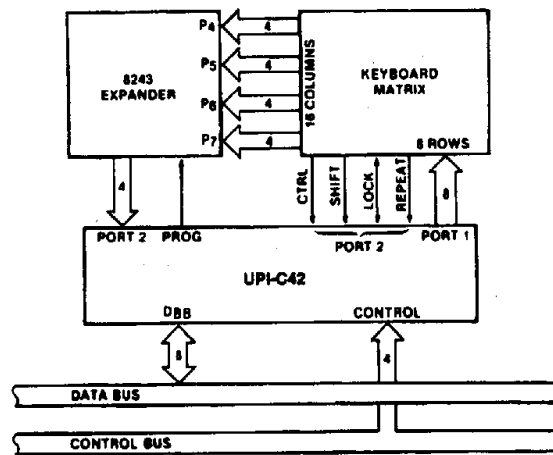
Figure 10. UPI-C42-8243 Keyboard Scanner
