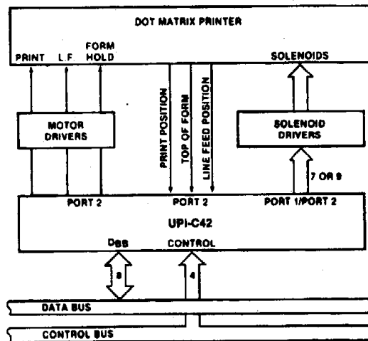
Figure 11. UPI-C42 80-Column Matrix Printer Interface
