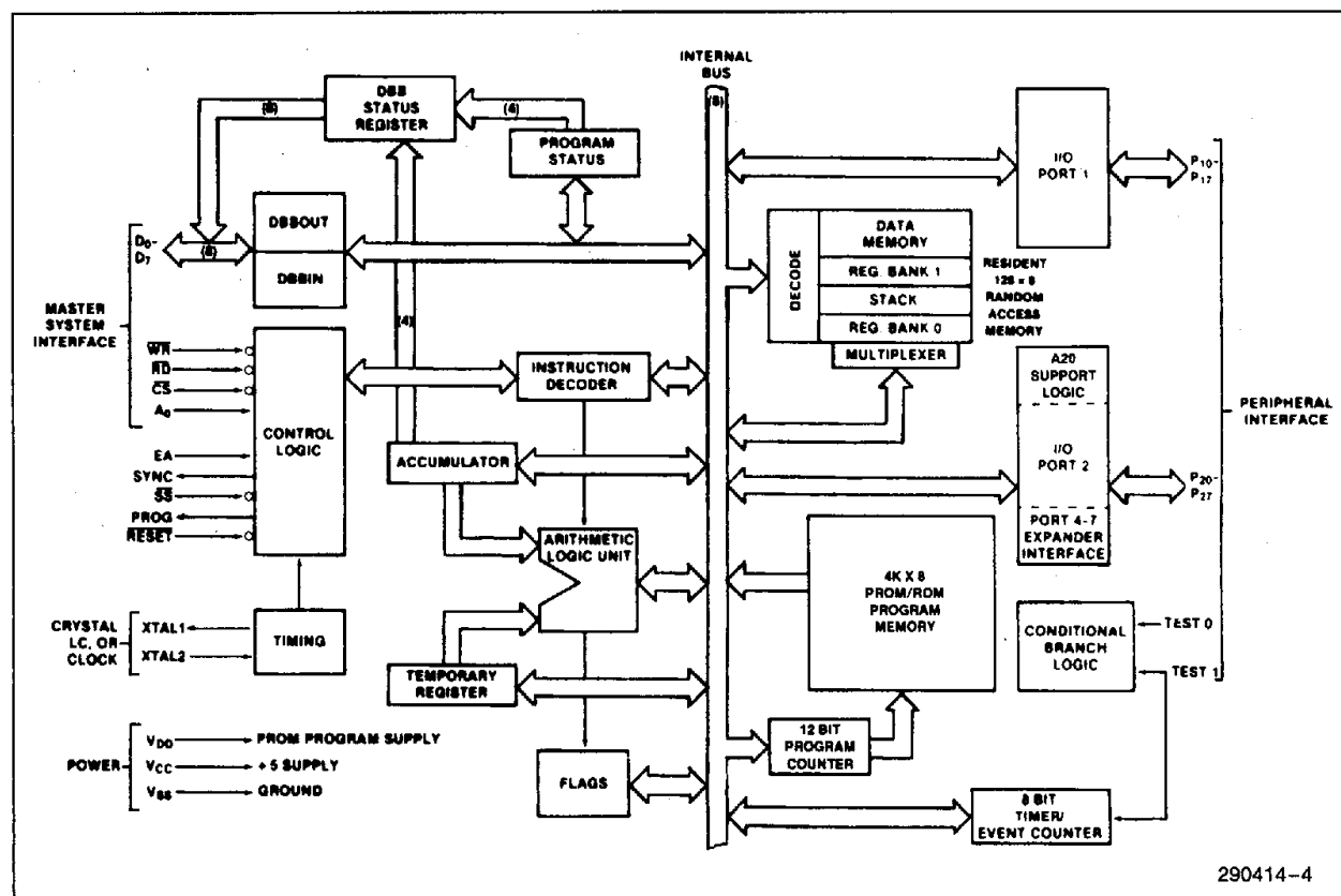
Figure 4. Block Diagram
