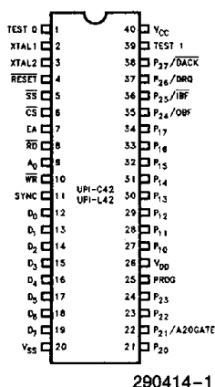
290414-1 Figure 1. DIP Pin Configuration
