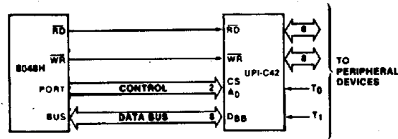
Figure 9. 8048H-UPI-C42 Interface
