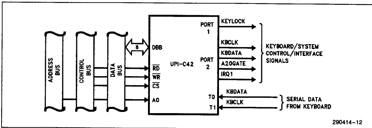
Figure 7. UPI-C42 Keyboard Controller
