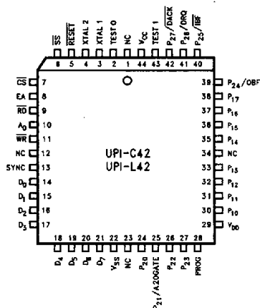
290414-2 Figure 2. PLCC Pin Configuration
