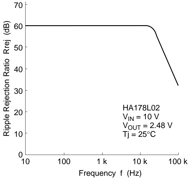
Ripple Rejection Ratio vs. Frequency (1)
