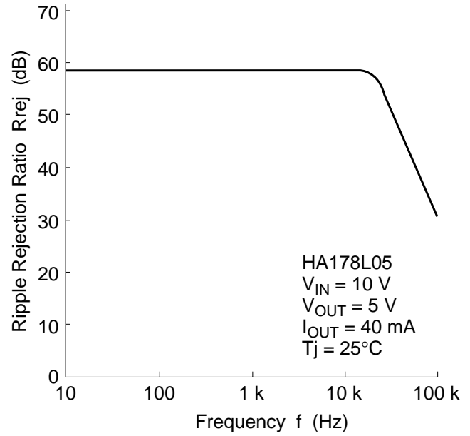
Ripple Rejection Ratio vs. Frequency (2)
