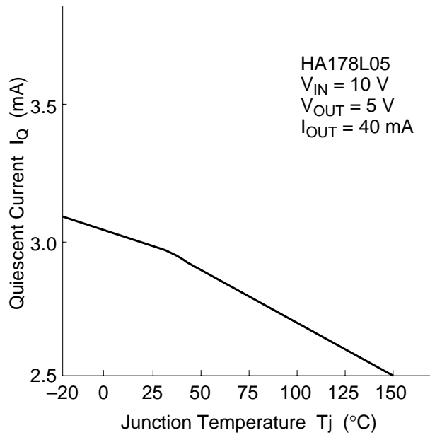
Quiescent Current vs. Junction Temperature (2)
