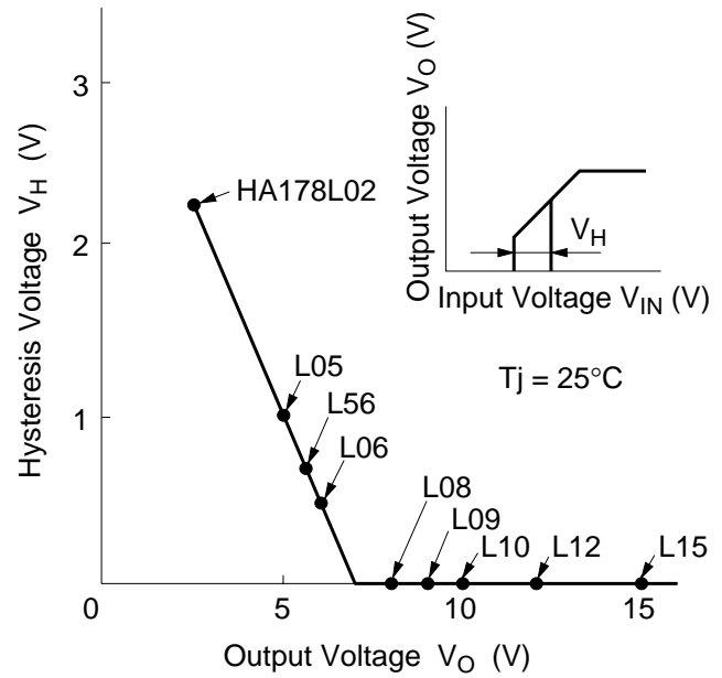
Hysteresis Voltage vs. Output Voltage
