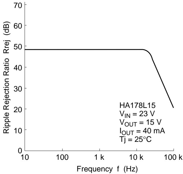
Ripple Rejection Ratio vs. Frequency (3)
