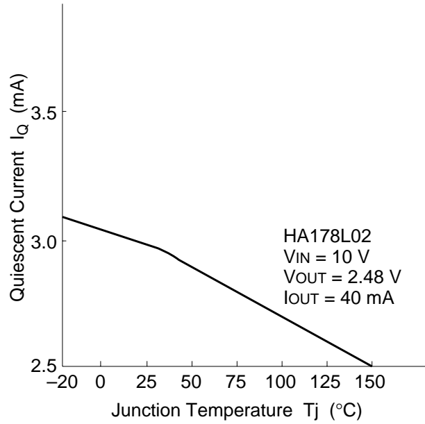
Quiescent Current vs. Junction Temperature (1)
