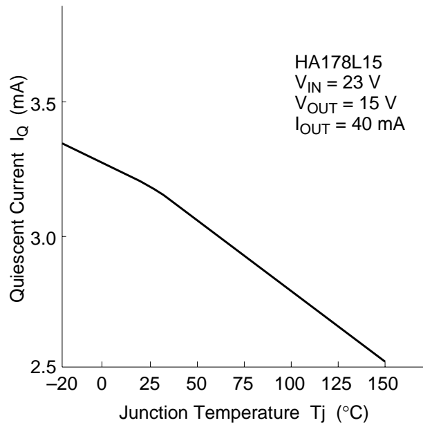
Quiescent Current vs. Junction Temperature (3)
