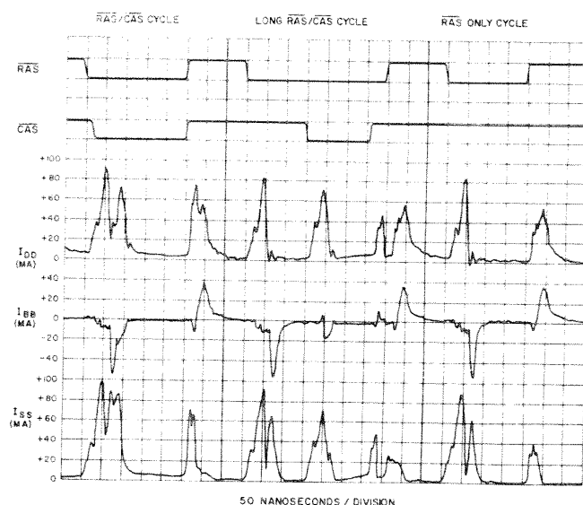
Fig. 5 Typical Current Waveforms
