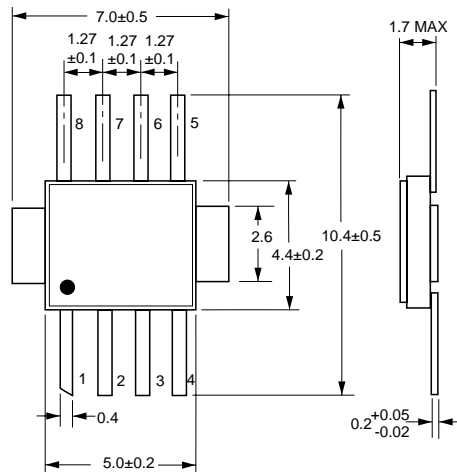
UPB582B PACKAGE OUTLINE BF08
