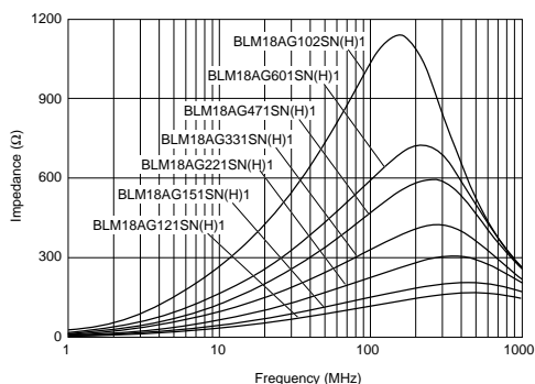
BLM18A Series
