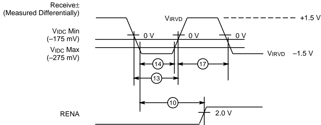
Receive \pm Input Pulse Width Timing
