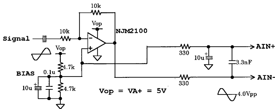
Fig. 2 Example of input buffer circuit (single end input)
