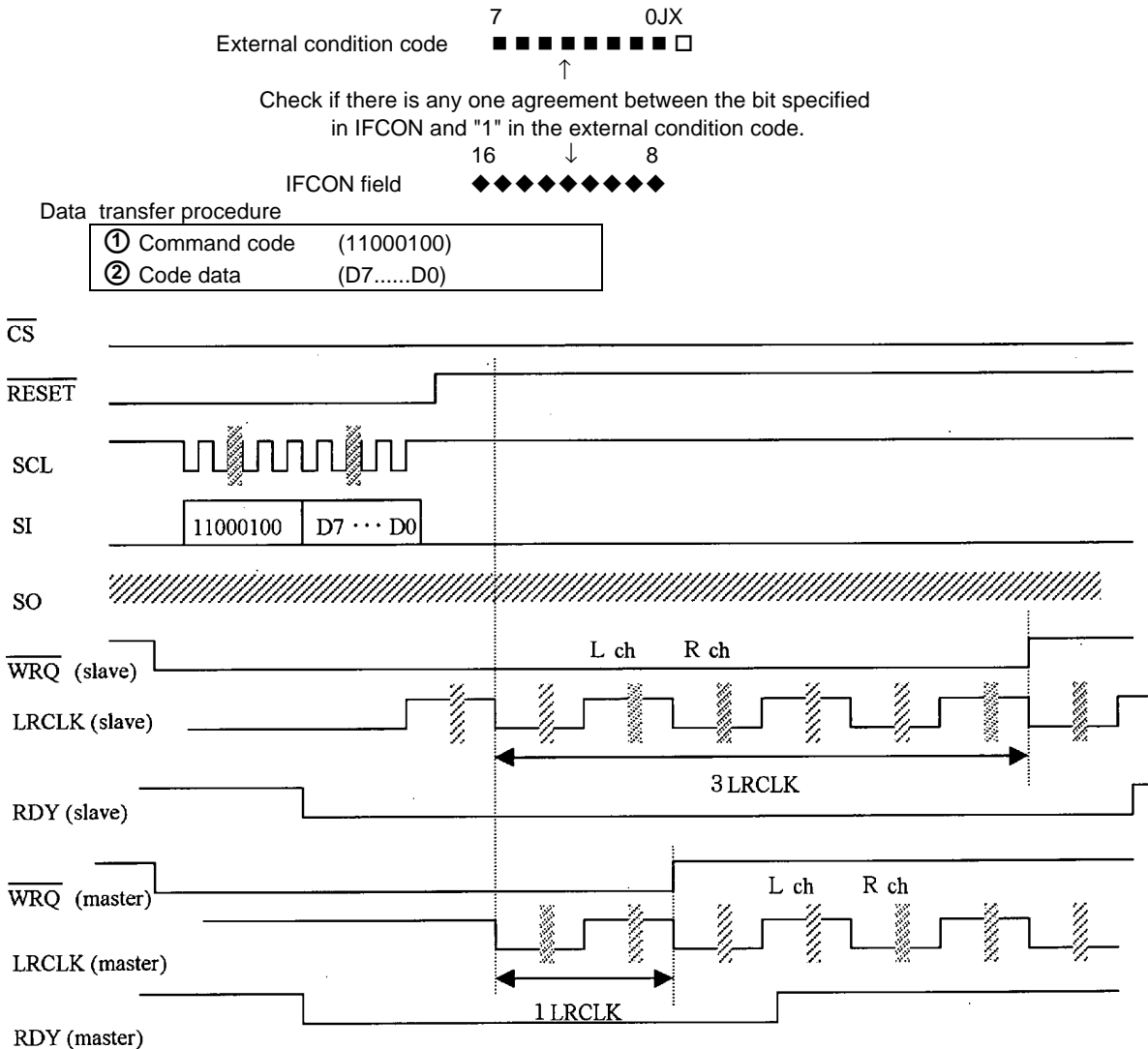
Timing for external conditional jump write operation (during reset phase)
