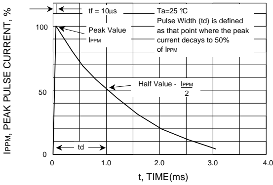
FIG.3 - PULSE WAVEFORM
