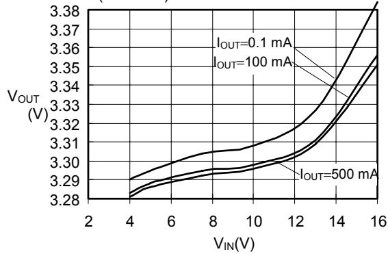
V_{OUT}-V_{IN} S-8521F33MC (Ta=25°C)
