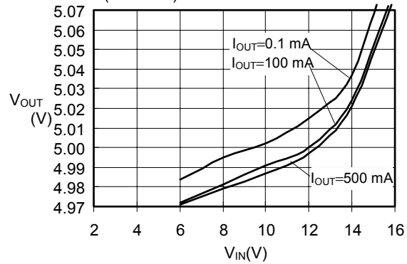
V_{OUT}-V_{IN} S-8521F50MC (Ta=25°C)
