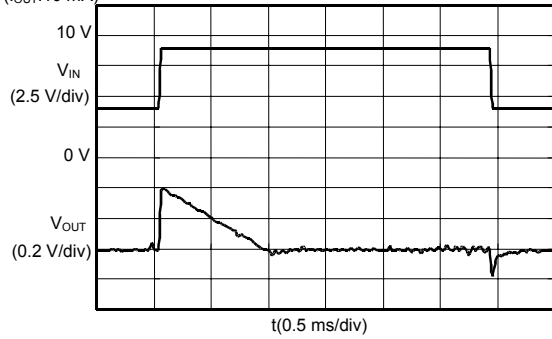
S-8520/1A30MC ( I_{OUT} :10 mA)
