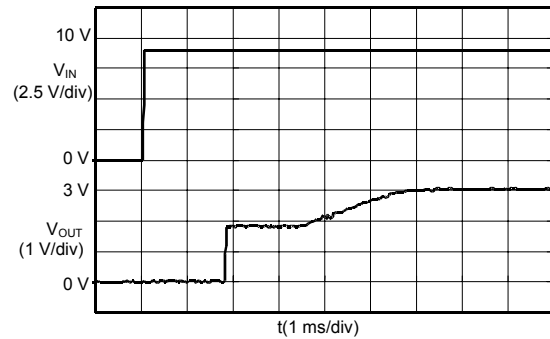
S-8520/1A30MC ( V_{IN} : 0 \rightarrow 9.0 V)
