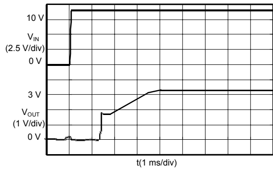
S-8520/1E33MC ( V_{IN} : 0 \rightarrow 9.0 V)
