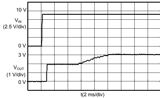
S-8520/1C30MC ( V_{IN} : 0 \rightarrow 9.0 V)
