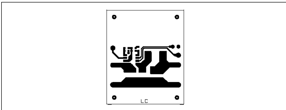
Figure 15. PCB layout (front side)
