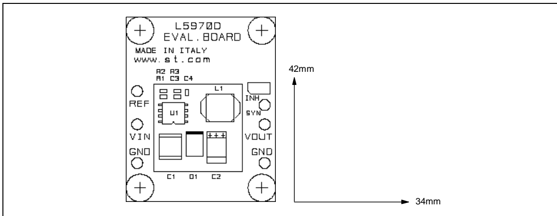
Figure 14. PCB layout (bottom side)
