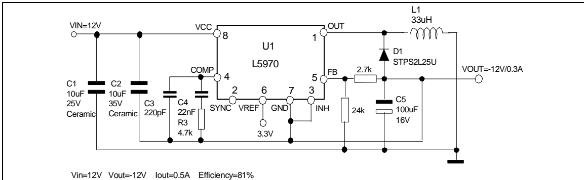
Figure 18. Positive Buck-Boost regul
