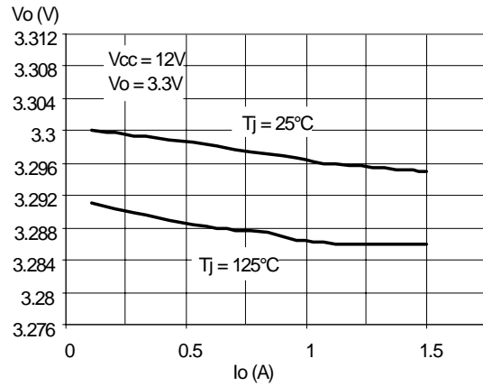
Figure 5. Line Regulation
