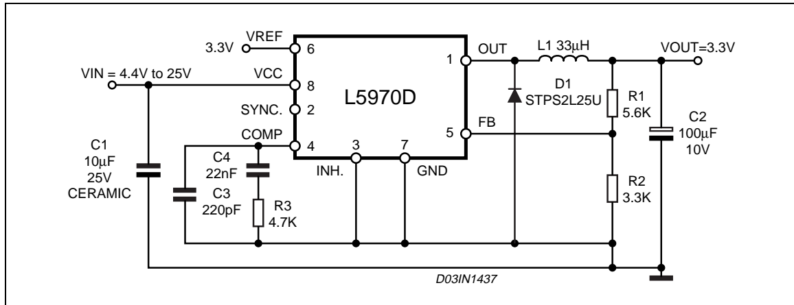
Figure 10. Demoboard schematic
