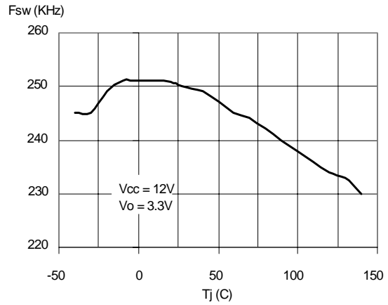
Figure 9. Switching Frequency vs. Junction Temperature
