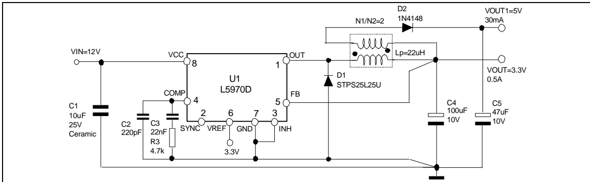
Figure 17. Buck-Boost regulator
