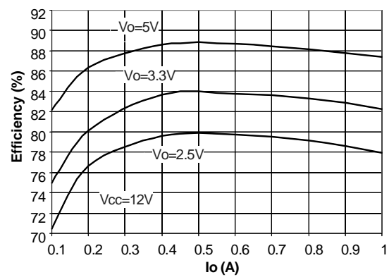
Figure 12. Efficiency vs. Output Current
