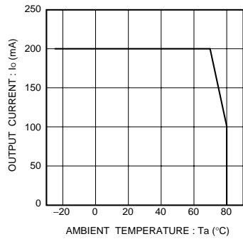
Fig.9 Derating curve
