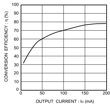
Fig.12 Conversion efficiency
