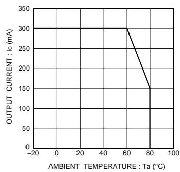
Fig.5 Derating curve
