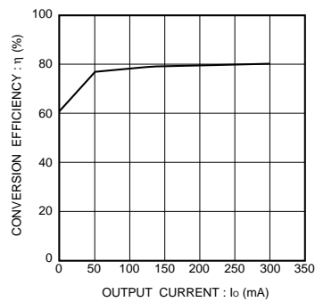
Fig.8 Conversion efficiency
