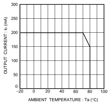
Fig.13 Derating curve
