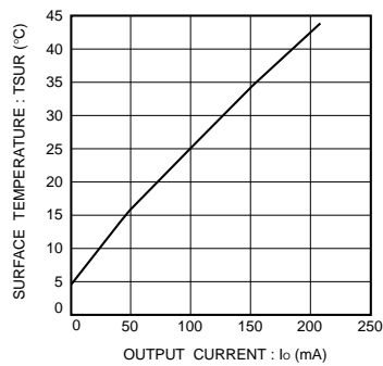
Fig.14 Surface temperature rise
