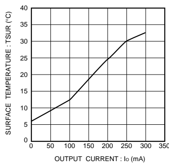
Fig.6 Surface temperature rise
