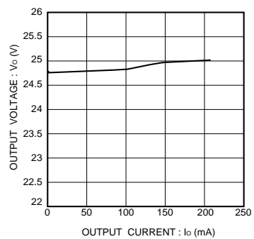
Fig.15 Output characteristic
