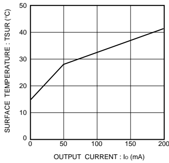
Fig.10 Surface temperature rise
