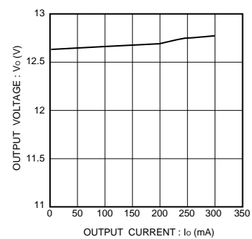
Fig.7 Output characteristic
