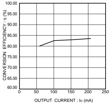
Fig.16 Conversion efficiency
