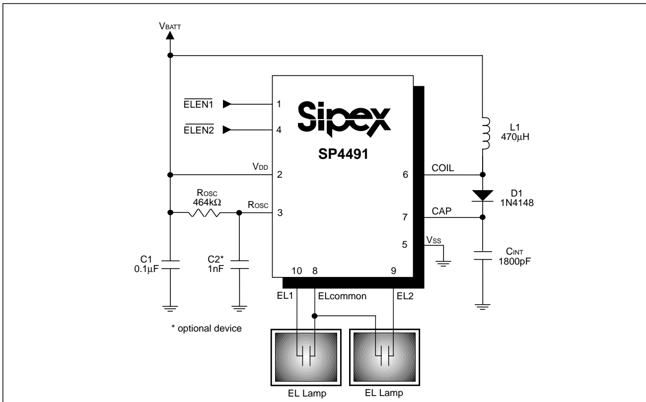
Figure 2: Typical Application Circuit of SP4491
