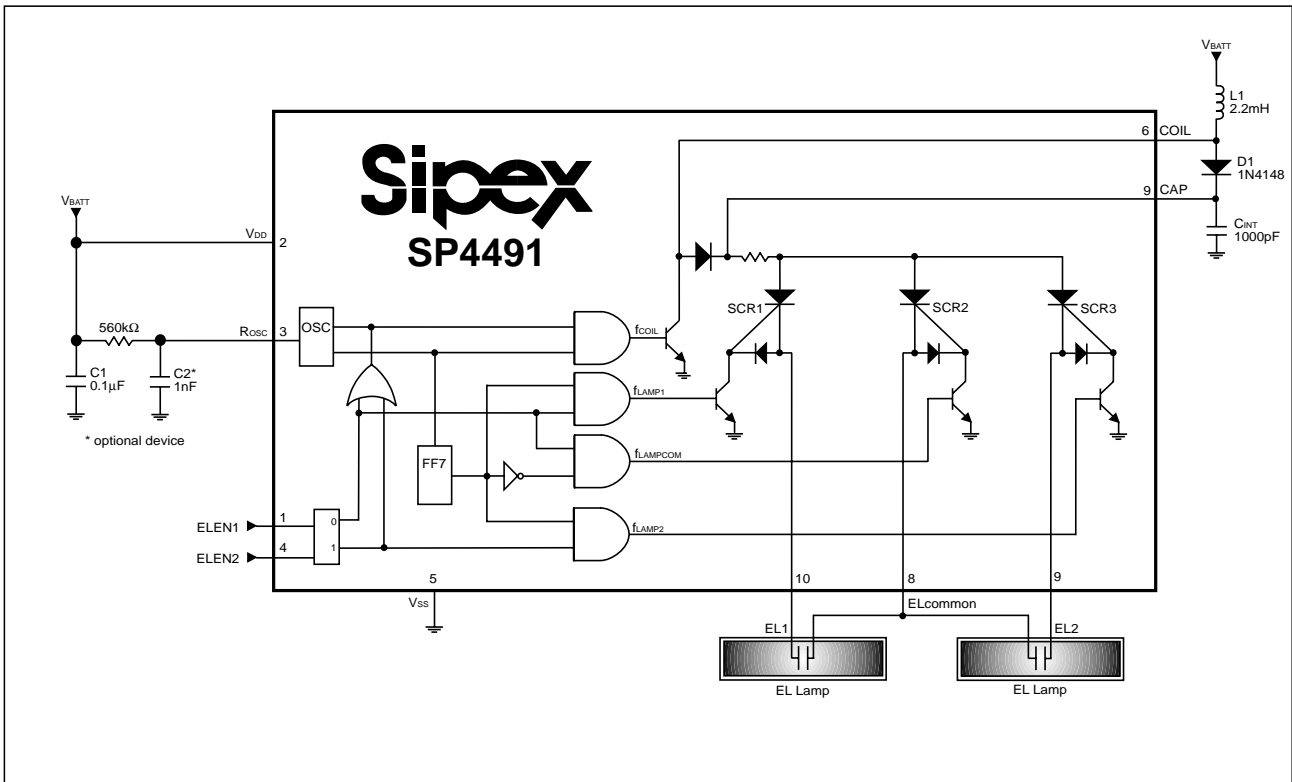
Figure 1: Internal Block Diagram of SP4491
