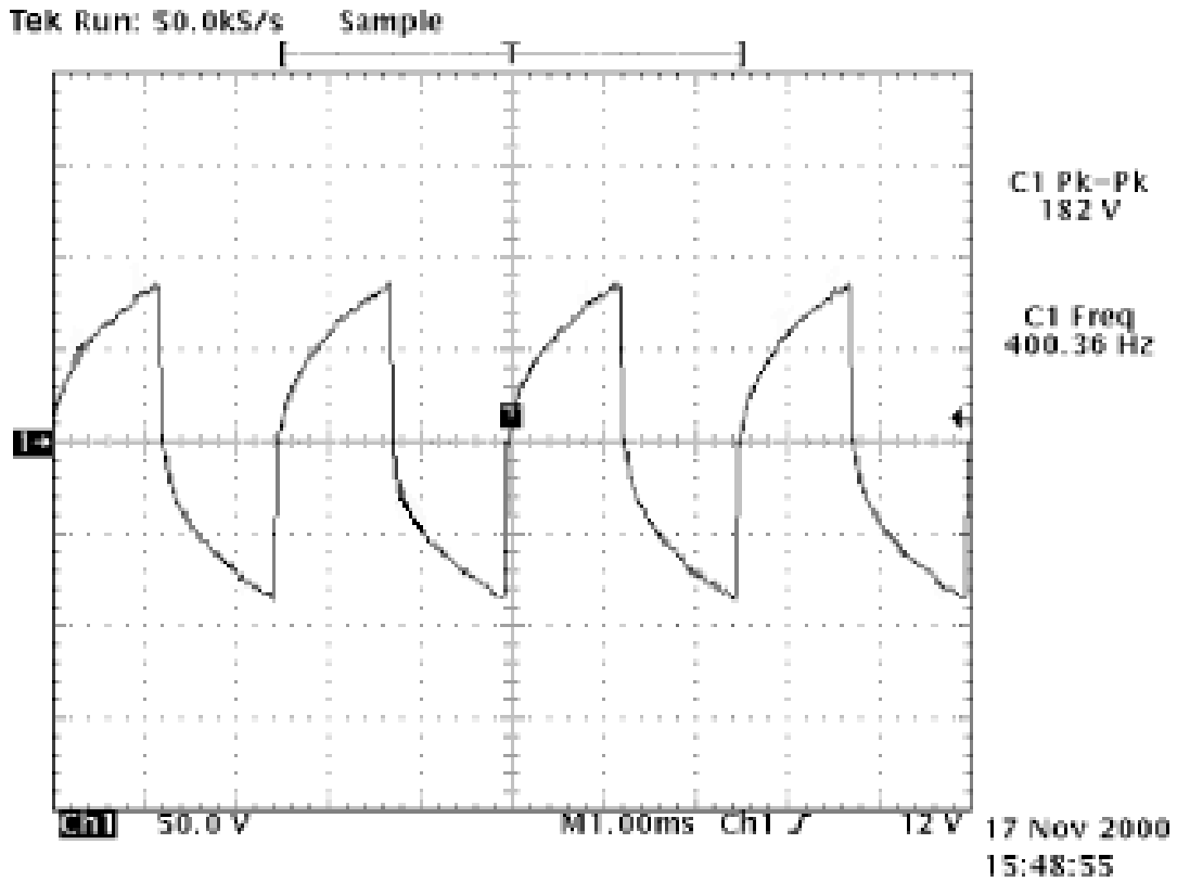
Figure 4: Typical EL Lamp Voltage Waveform
