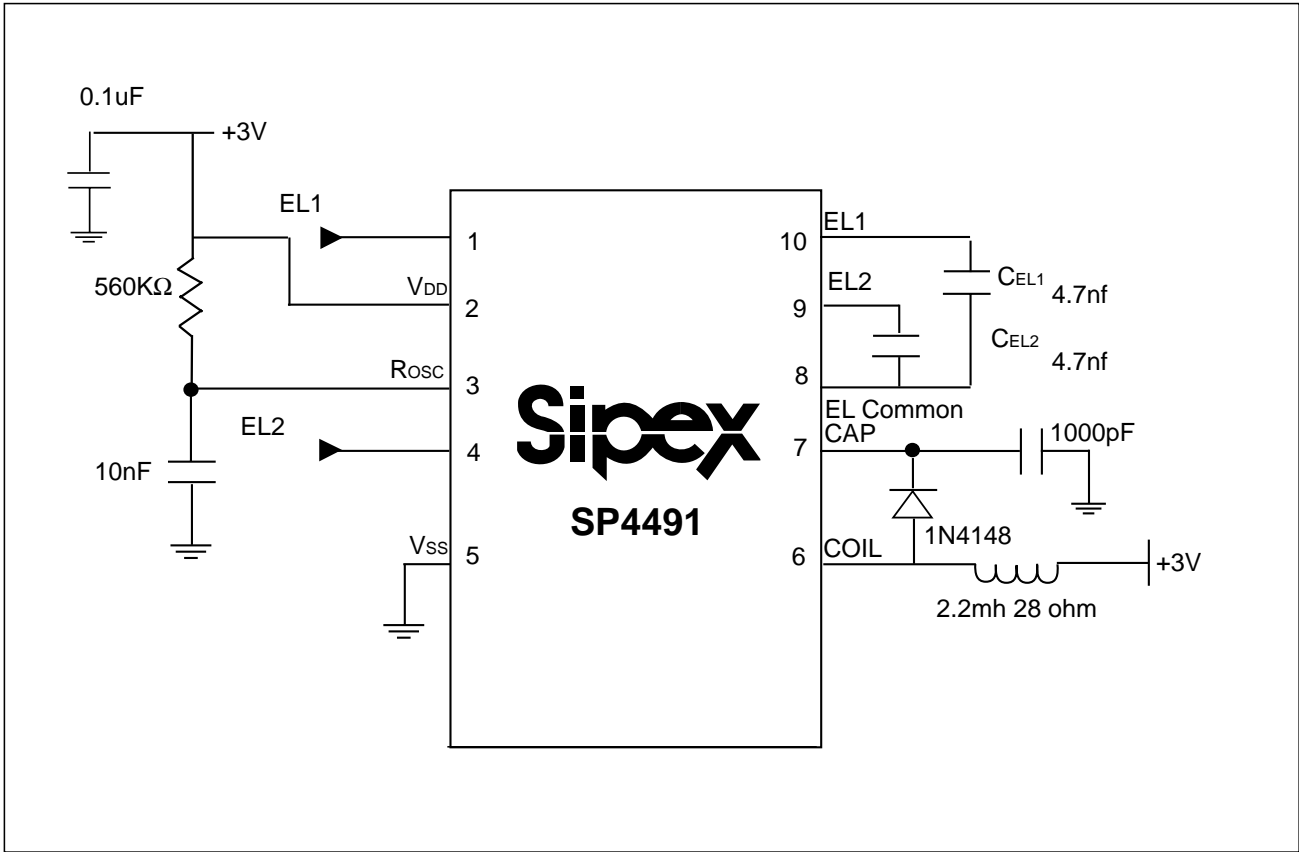
Figure 3: Test Circuit Diagram of SP4491
