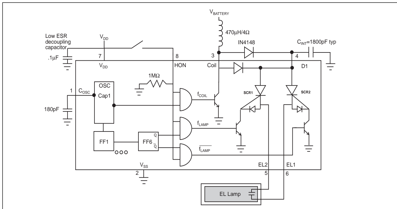
SP4425 Schematic
