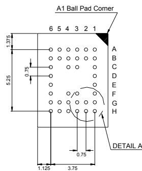
BOTTOM VIEW ( BALL SIDE )
