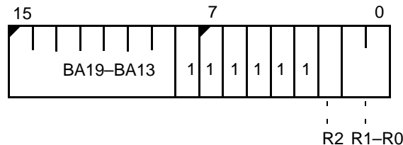
Figure 5-3 Midrange Memory Chip Select Register
