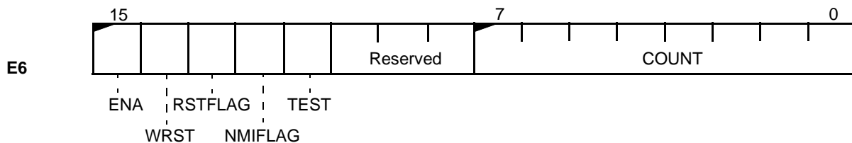
Watchdog Timer Control Register (WDTCN) Page 6-3
