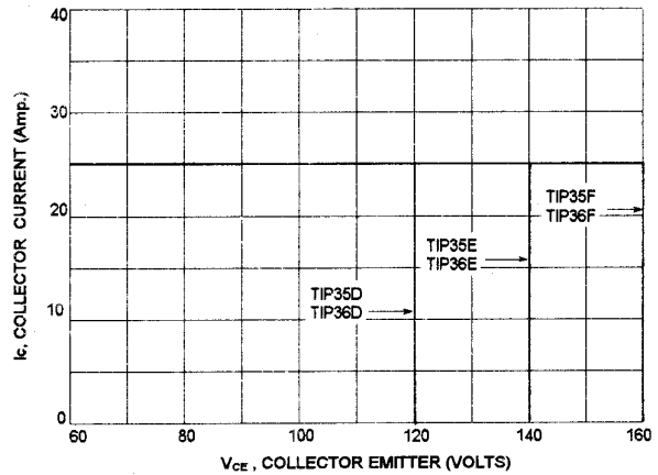
FIG-5 REVERSE BIASE SAFE OPERATING AREA
