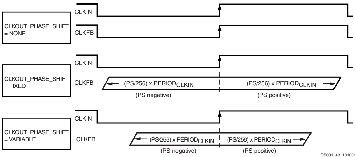
Figure 47: Fine-Phase Shifting Effects
