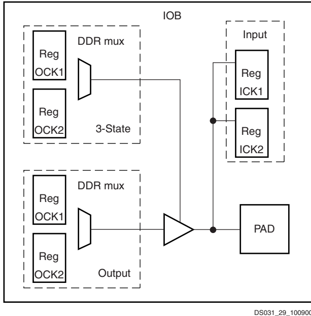
Figure 3: Virtex-II IOB Block
