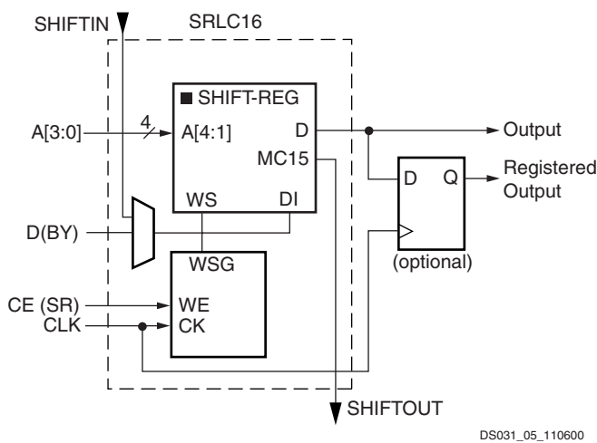
Figure 22: Shift Register Configurations
