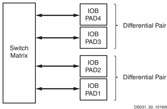
Figure 2: Virtex-II Input/Output Tile
