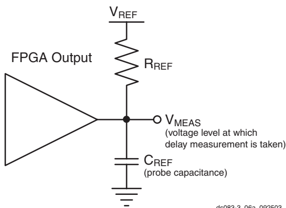
Figure 51: Generalized Test Setup
