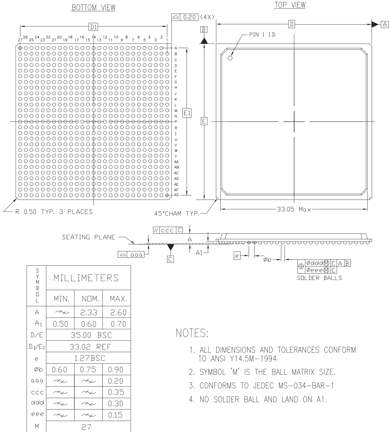
Figure 54: BG728 Standard BGA Package Specifications
