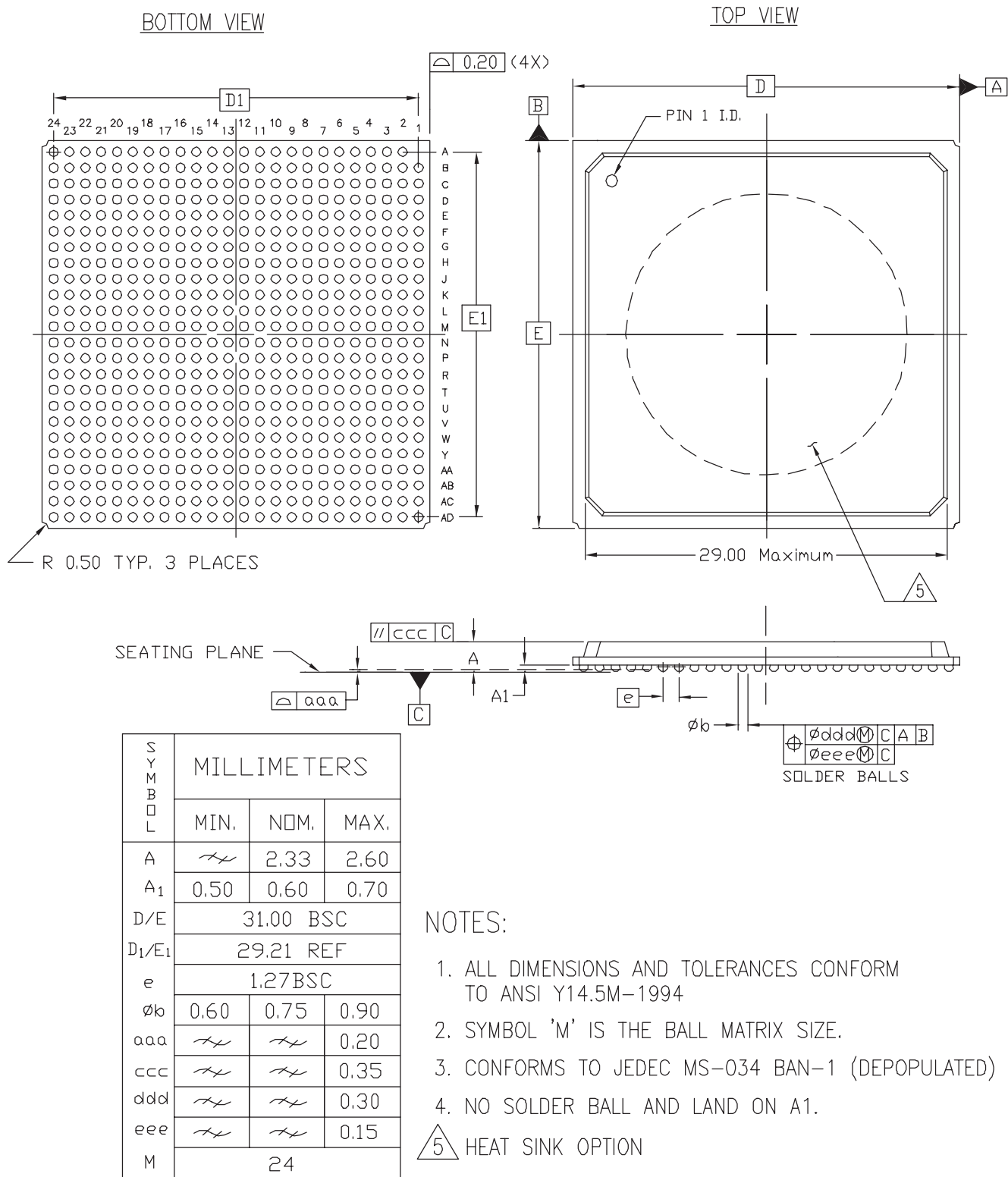
Figure 53: BG575 Standard BGA Package Specifications
