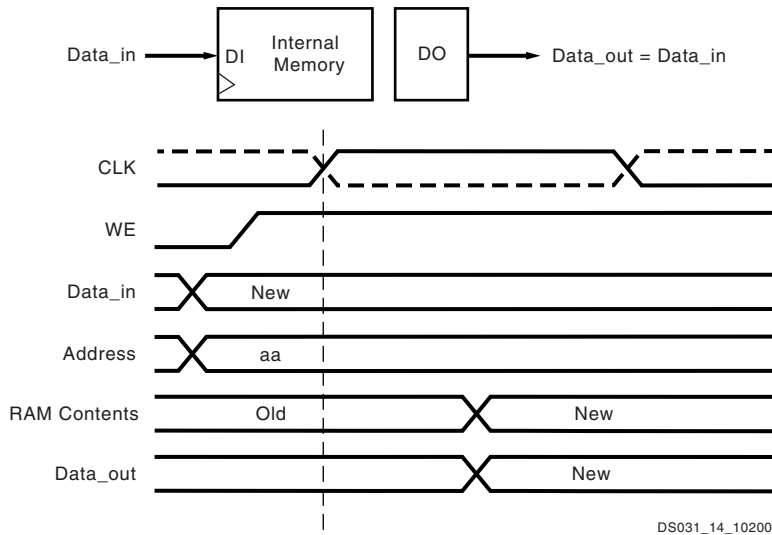
Figure 32: WRITE_FIRST Mode
