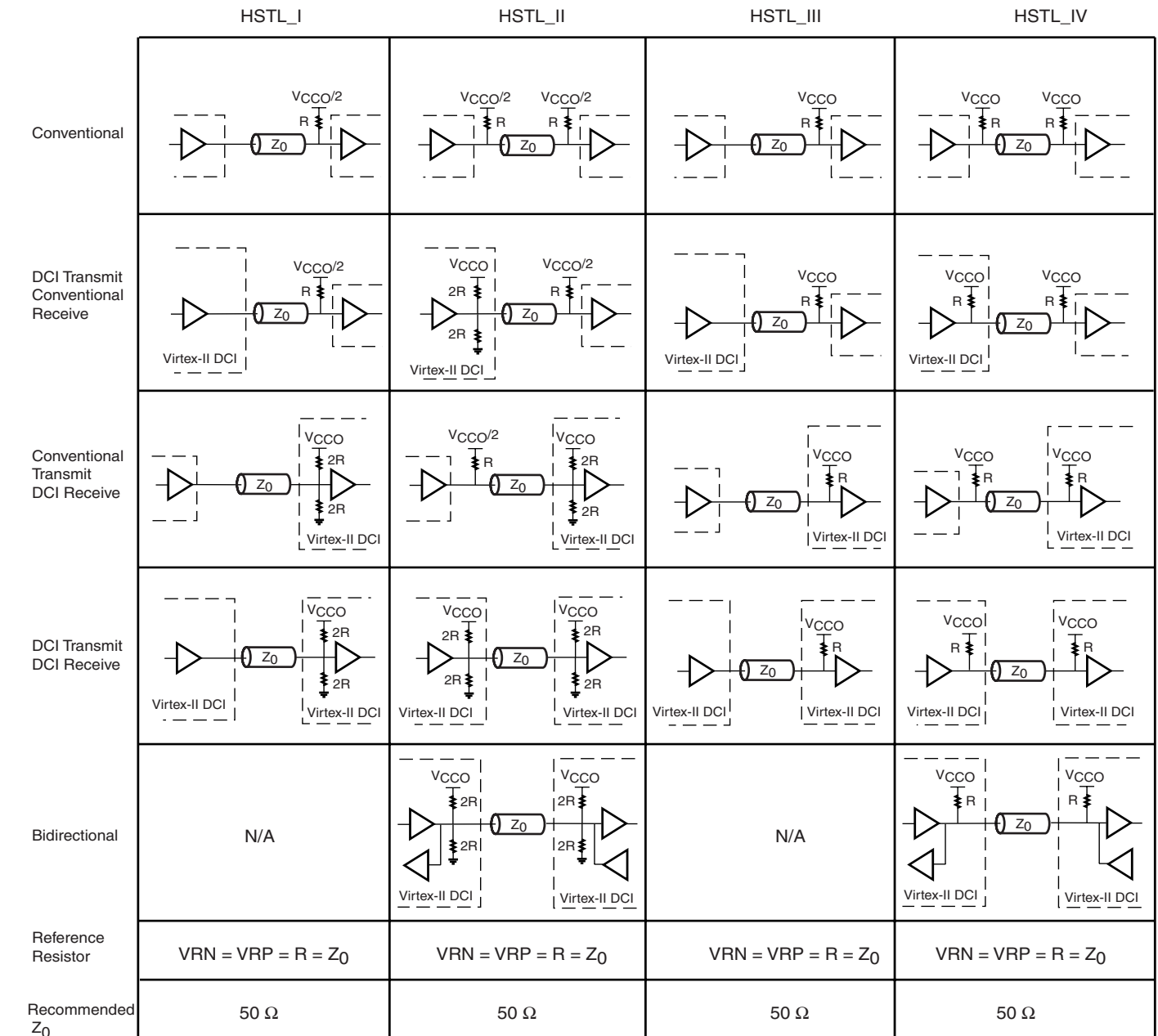
Figure 12: HSTL DCI Usage Examples
