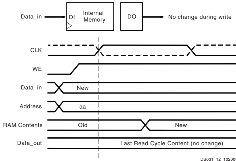
Figure 34: NO_CHANGE Mode
