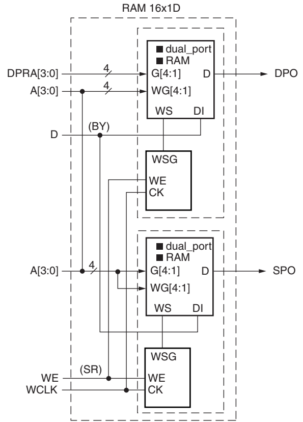
Figure 21: Dual-Port Distributed SelectRAM (RAM16x1D)
