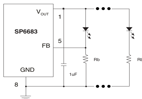
Figure 9. Driving discrete white LEDs as current source
