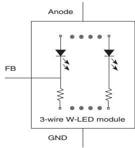
Fig 10. 3-wire white LED module
