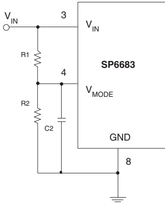
Figure 13. Programming the Vmode Resistors
