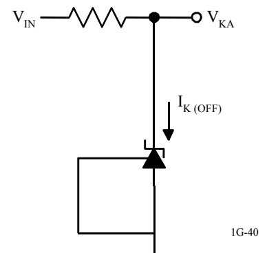
TEST CIRCUIT For I_{K(OFF)}
