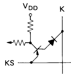
Transistor switch
