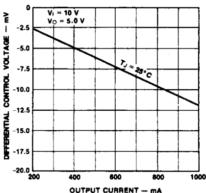
Differential Control Voltage vs Output Current
