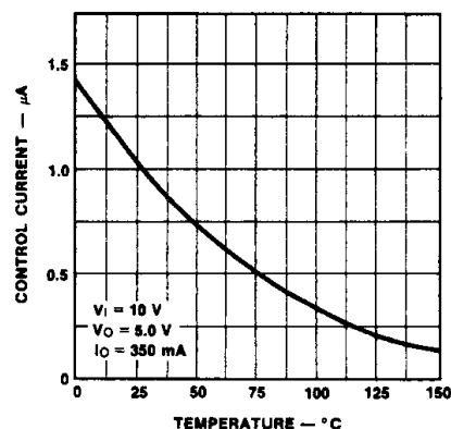
Control Current vs Temperature
