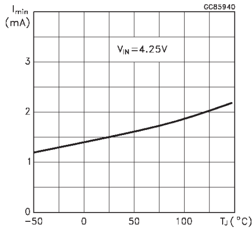
Minimum Load Current vs Temperature
