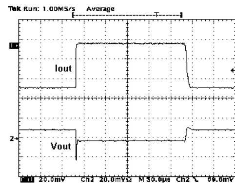
Figure 28 : Load Transient
