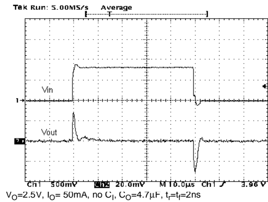
Figure 11 : Line Transient
