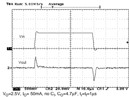
Figure 12 : Line Transient
