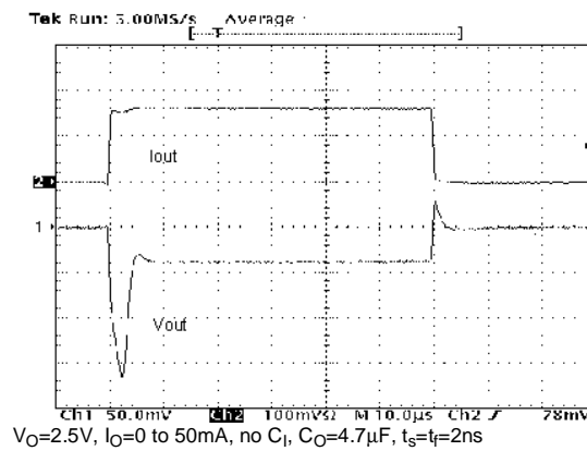
Figure 14 : Load Transient
