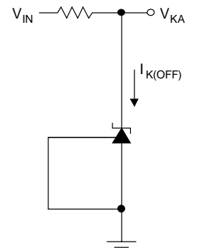
TEST CIRCUIT 3
