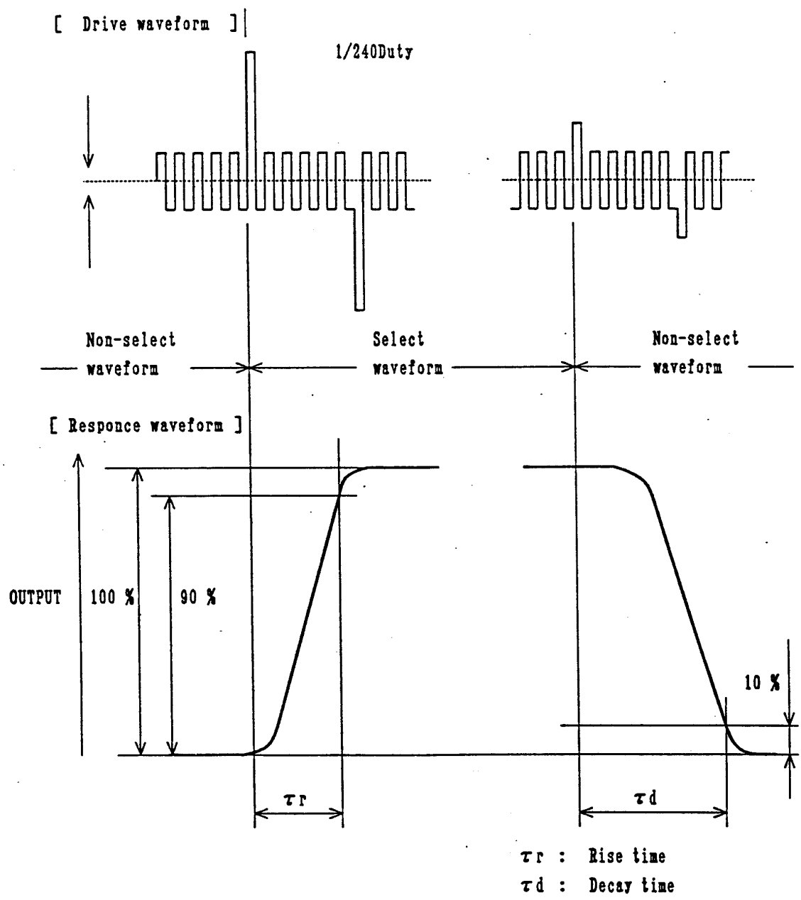
Fig.8 Difinition of Response Time
