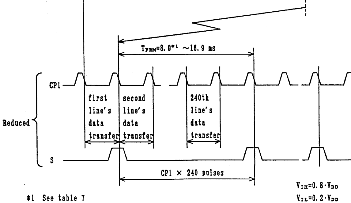
Fig. 3 Interface timing chart
