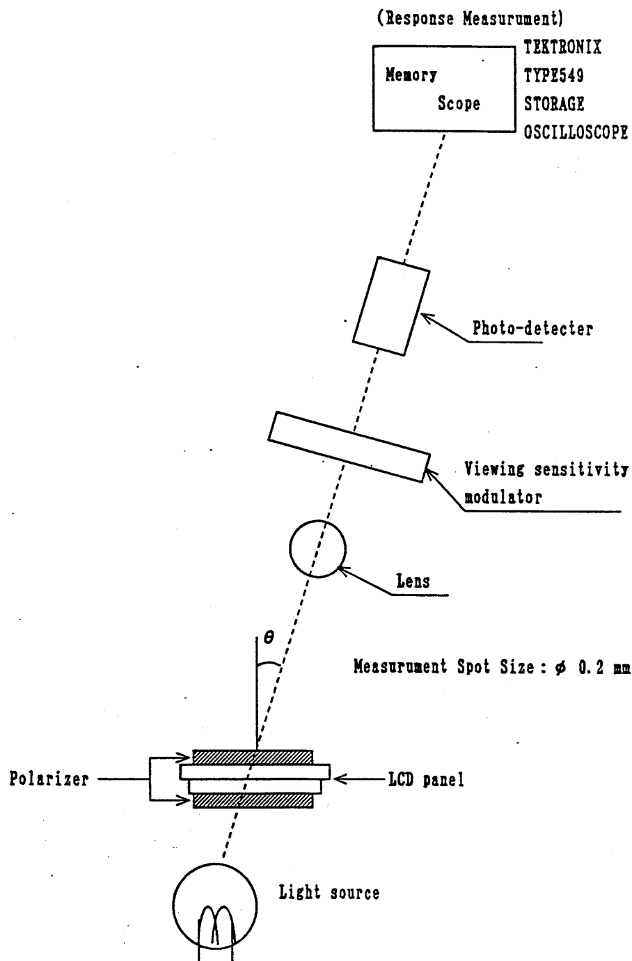
Fig.7 Optical Characteristics Test Method II
