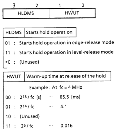
Hold operating mode command register (Port address: OP10, Initial value: *0**)
