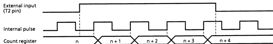
Figure 3-11. Pulse Width Measurement Mode Timing Chart
