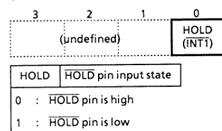
Hold operating mode status register (Port address: IPOE)
