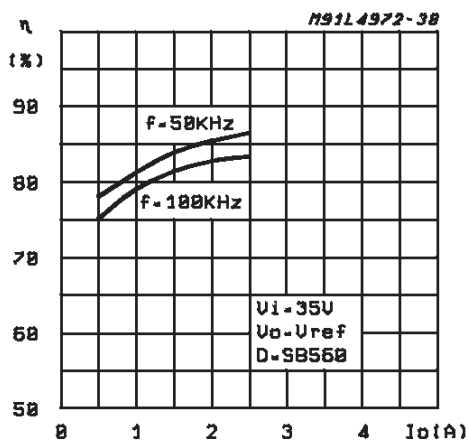
Figure 32 : Efficiency vs. Output Current.
