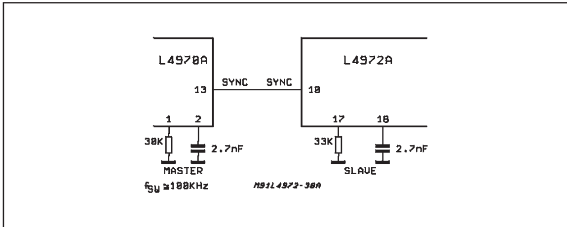
Figure 41 : L4972A's Sync. Example.
