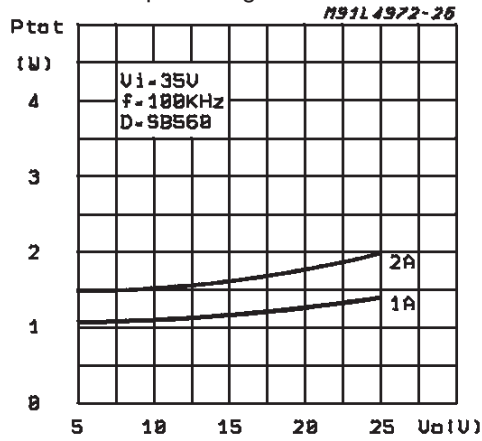
Figure 28 : Power Dissipation (device only) vs. Output Voltage.
