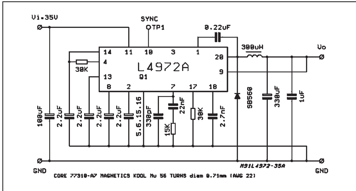
Figure 39 : 2A – 5.1V Low Cost Application Circuit.
