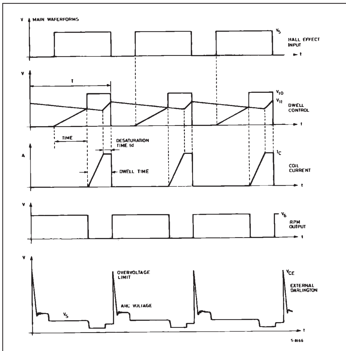
Figure 1 : Main Waveforms.
