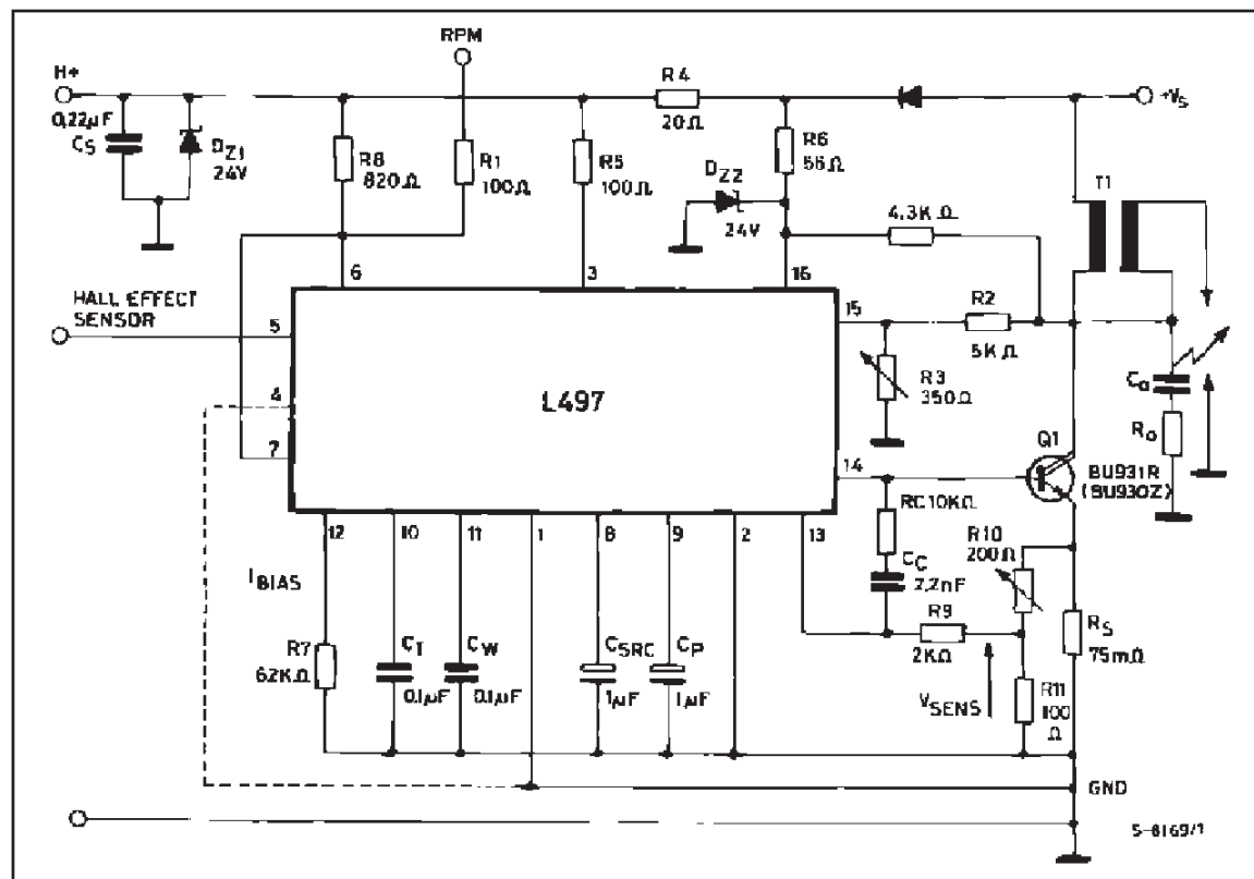
Figure 4 : Application Circuit.
