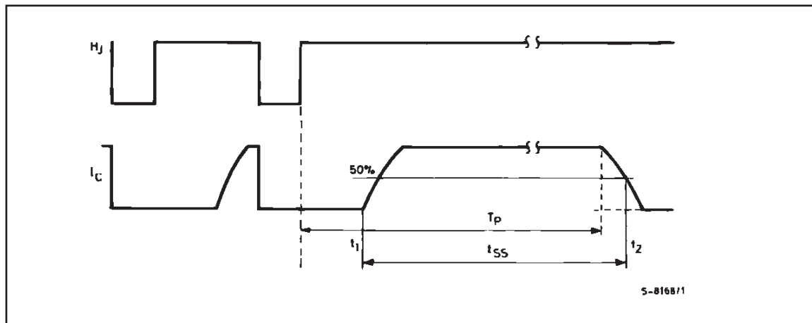
Figure 3 : Permanent Conduction Protection.
