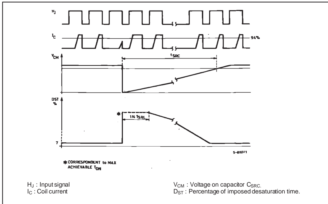
Figure 3 : Permanent Conduction Protection.
