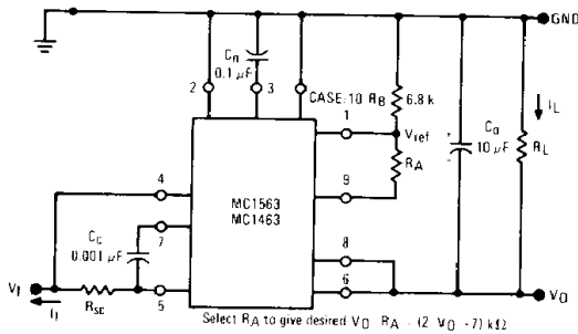
FIGURE 6 - LOAD REGULATION
