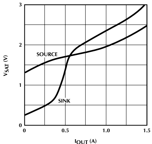
Figure 8. Saturation Curves
