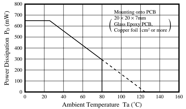
P_D - T_a (AN8000M Series)
