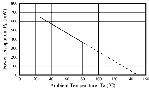
P_D - T_a (AN8000 Series)
