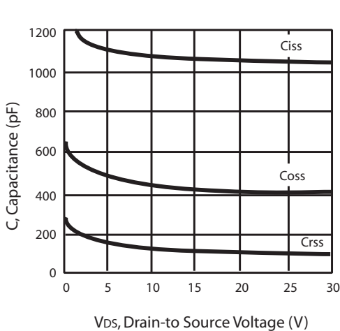
Figure 3. Capacitance
