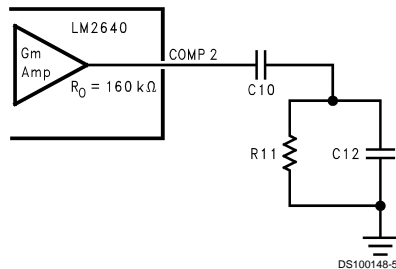
FIGURE 4. Typical Compensation Network
