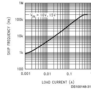
CH1 Skip Frequency vs Load Current
