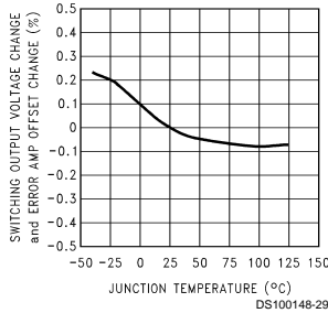
Normalized Error Amplifier Offset vs Junction Temperature
