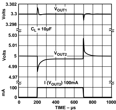
Figure 14. Load Transient on V_{\text{OUT}2} and Crosstalk on V_{\text{OUT}1} on ADP3302AR4 for 1 mA to 100 mA Pulse
