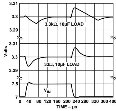
Figure 12. Line Transient Response (10 \mu\text{F} Load) on ADP3302AR4
