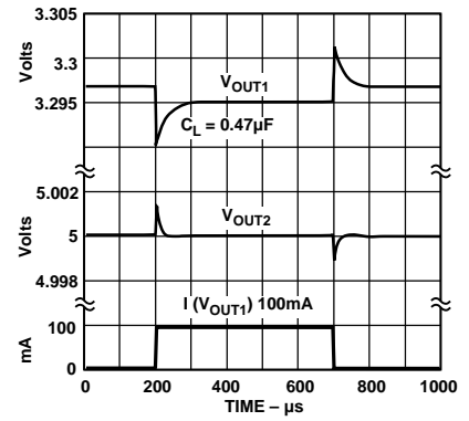
Figure 13. Load Transient on V_{\text{OUT}1} and Crosstalk of V_{\text{OUT}2} on ADP3302AR4 for 1 mA to 100 mA Pulse
