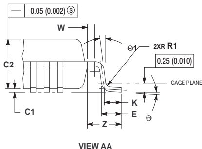
Figure 17-2 100-pin QFP mechanical dimensions
