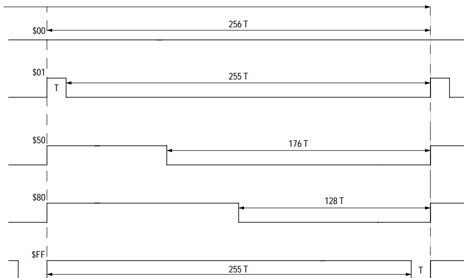
Figure 12-2 PWM output waveforms (POL = 1, active high)
