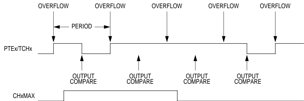
Figure 11-7. CHxMAX Latency
