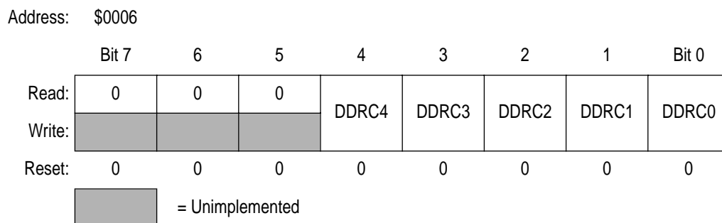
Figure 12-8. Data Direction Register C (DDRC)
