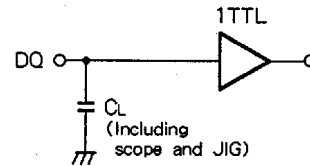
Fig.1 Output load
