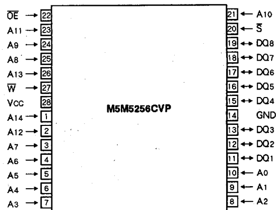
Outline 28P2C-A
