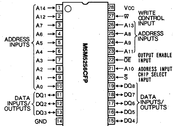
Outline 28P2W-C
