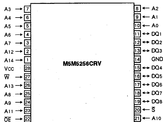
Outline 28P2C-B
