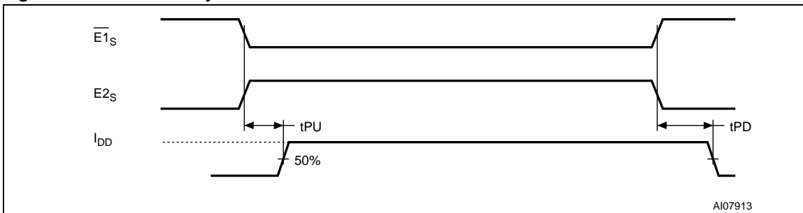
Figure 19. SRAM Standby AC Waveforms
