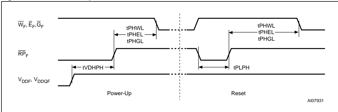
Figure 15. Flash Power-Up and Reset AC Waveforms
