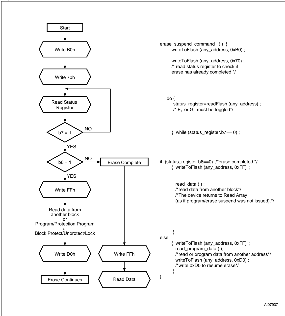
Figure 30. Erase Suspend & Resume Flowchart and Pseudo Code
