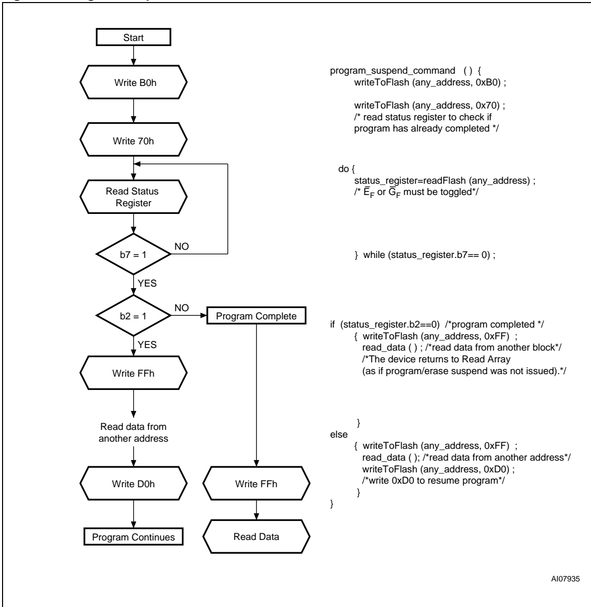
Figure 28. Program Suspend & Resume Flowchart and Pseudo Code
