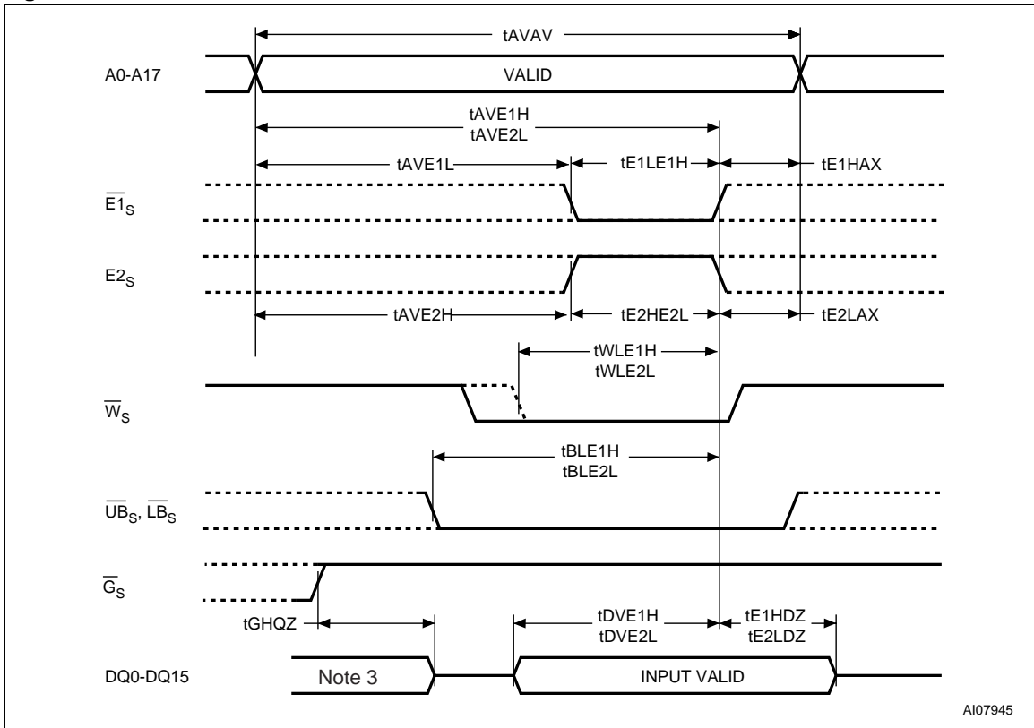
Figure 21. SRAM Write AC Waveforms, \overline{E1}_S Controlled
