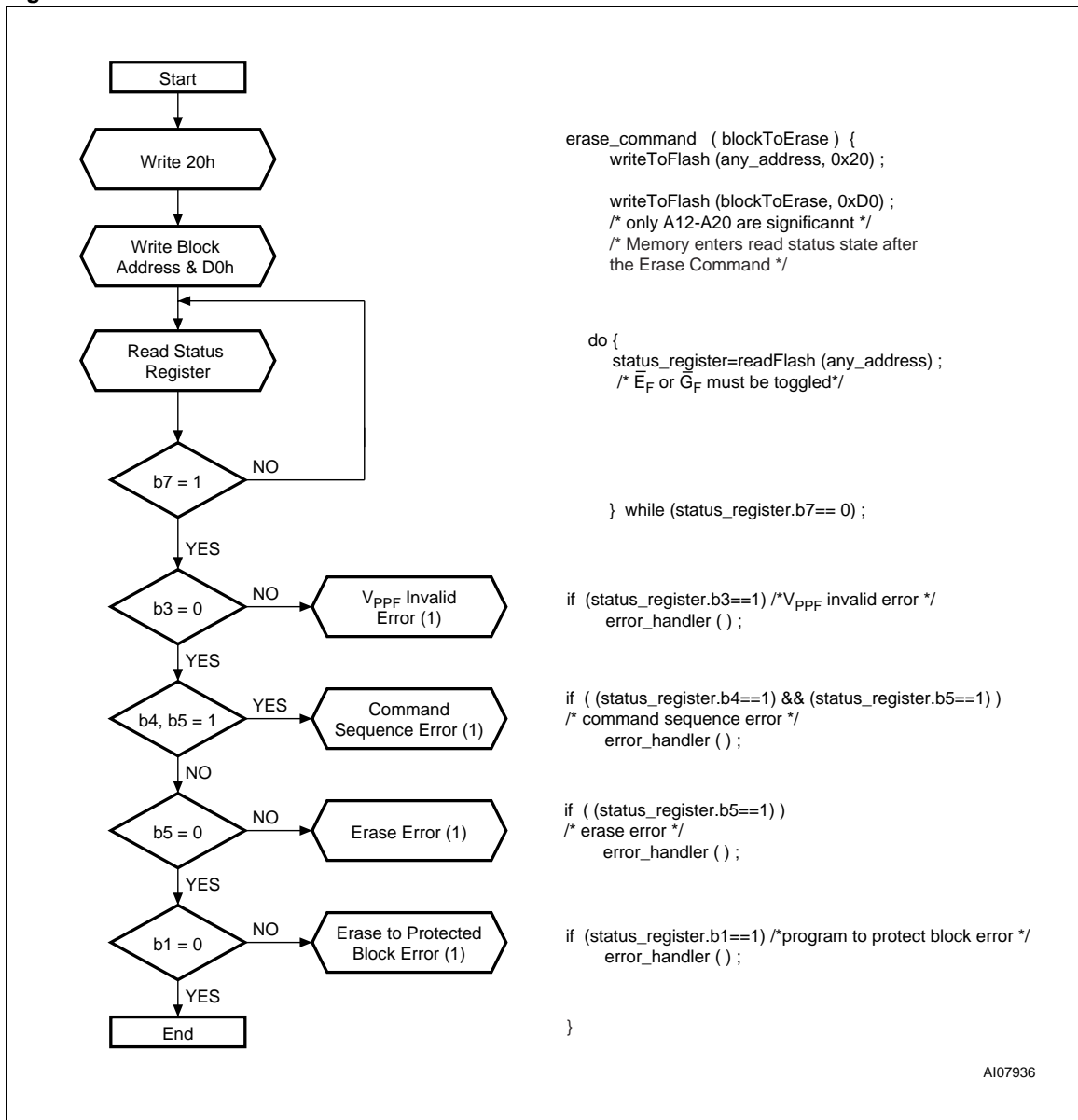
Figure 29. Erase Flowchart and Pseudo Code
