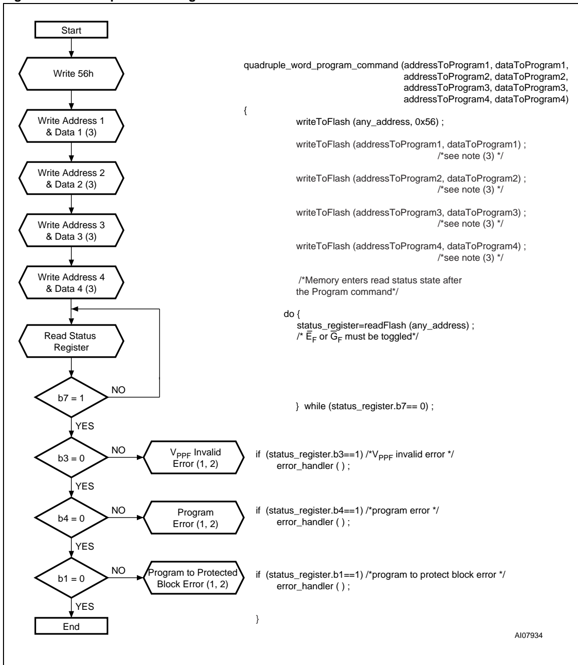
Figure 27. Quadruple Word Program Flowchart and Pseudo Code
