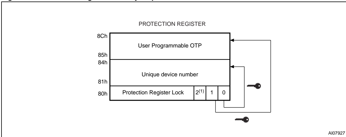
Figure 11. Protection Register Memory Map
