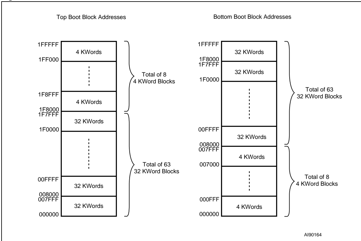
Figure 10. Flash Block Addresses
