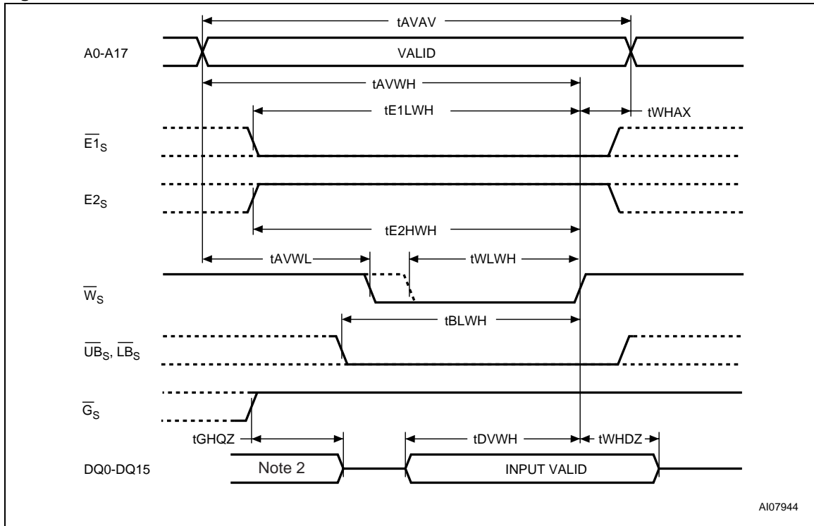
Figure 20. SRAM Write AC Waveforms, \overline{W}_S Controlled
