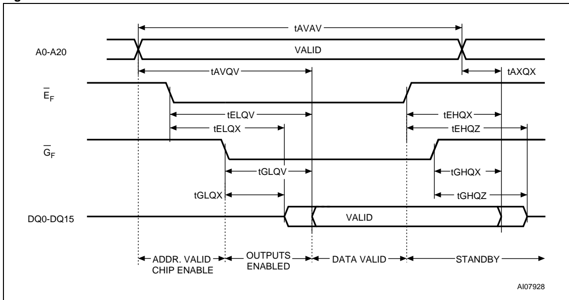
Figure 12. Flash Read Mode AC Waveforms
