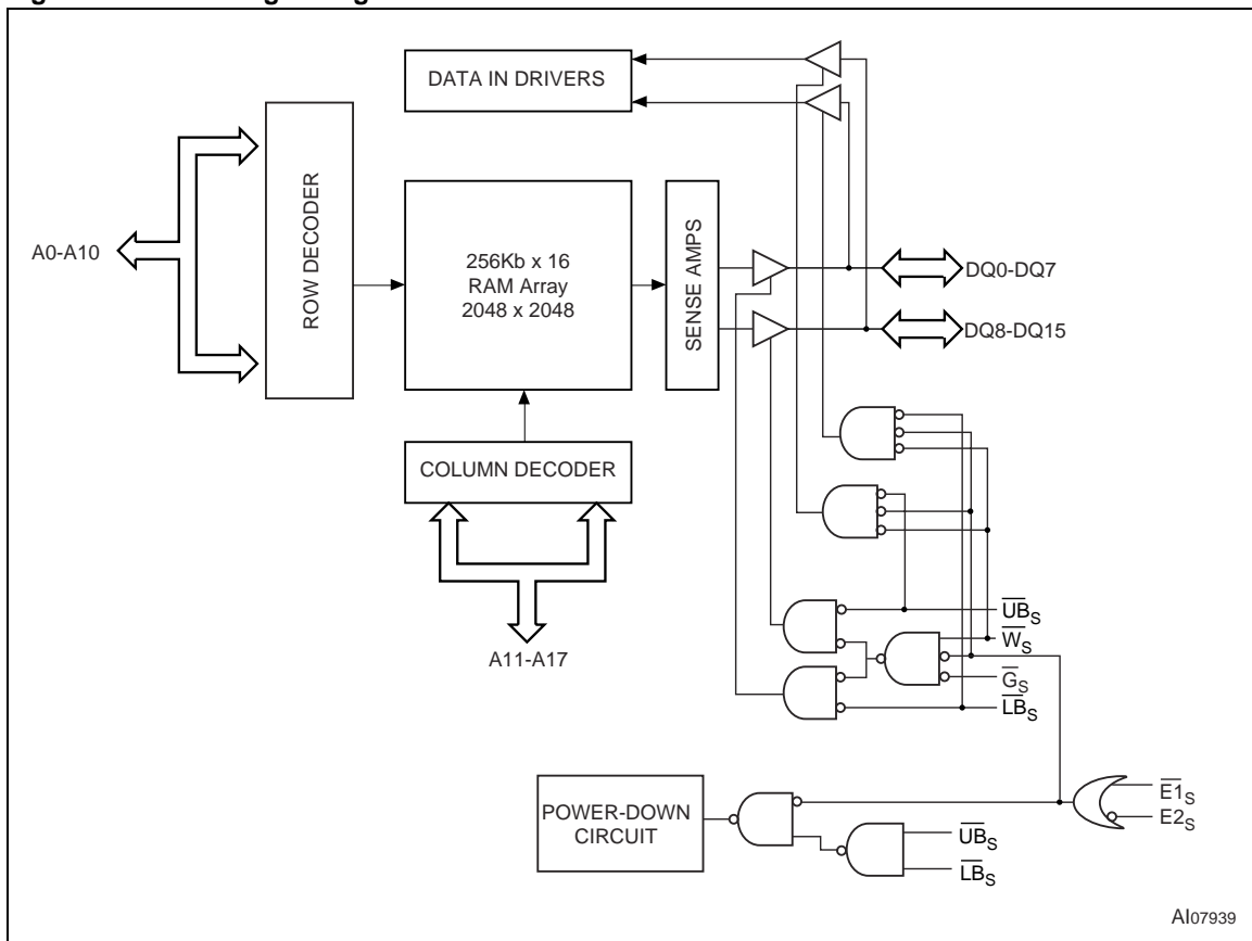
Figure 16. SRAM Logic Diagram
