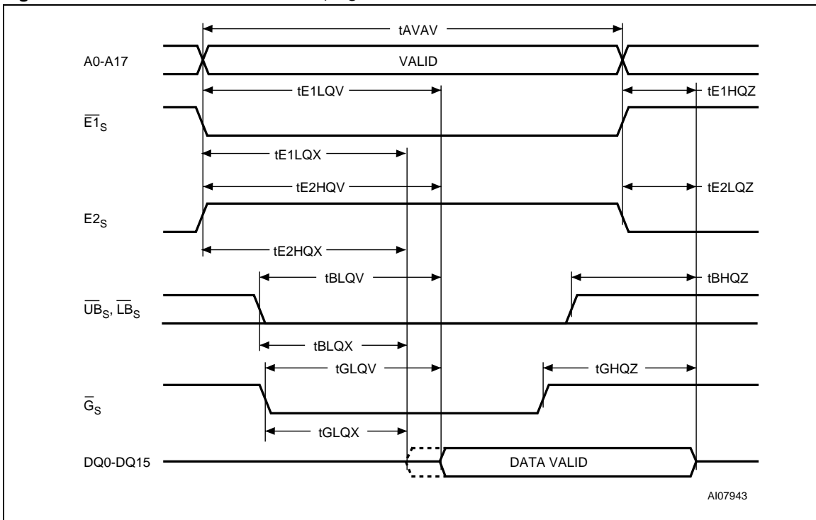
Figure 18. SRAM Read AC Waveforms, \overline{G}_S Controlled
