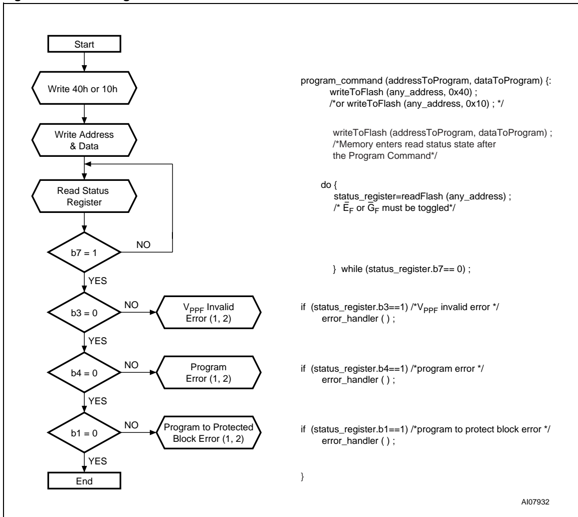
Figure 25. Flash Program Flowchart and Pseudo Code
