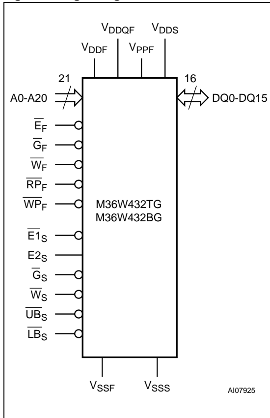
Figure 2. Logic Diagram
