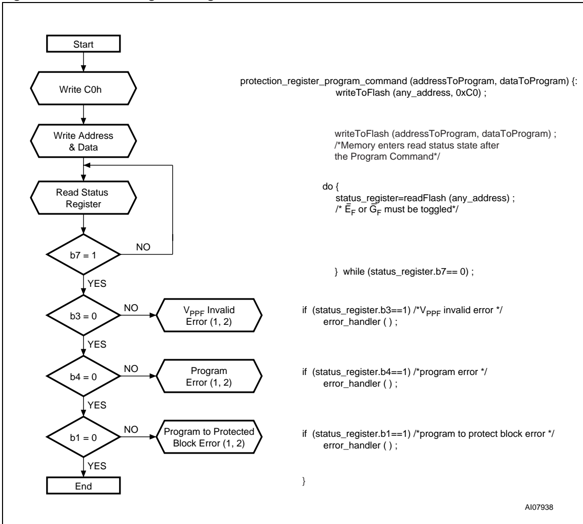
Figure 32. Protection Register Program Flowchart and Pseudo Code
