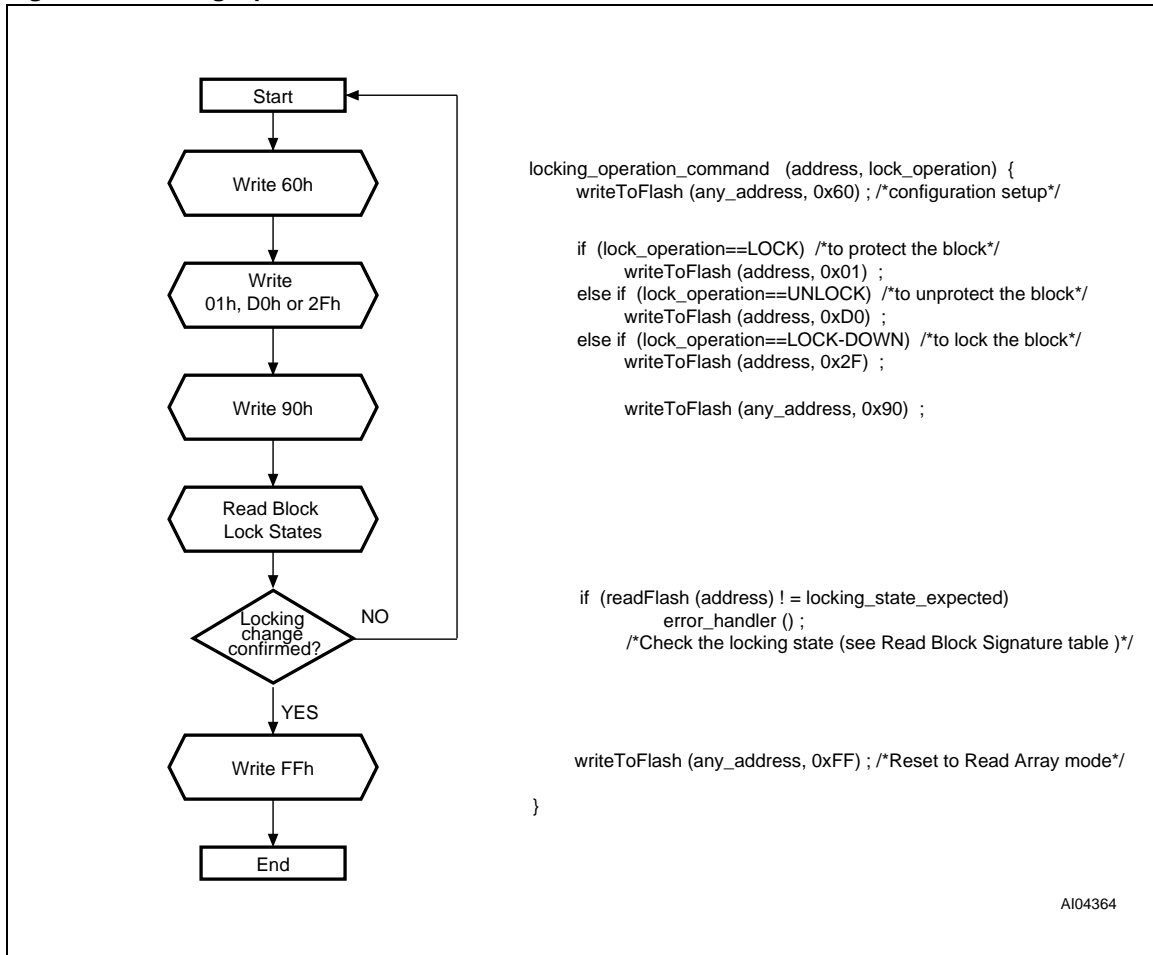
Figure 31. Locking Operations Flowchart and Pseudo Code
