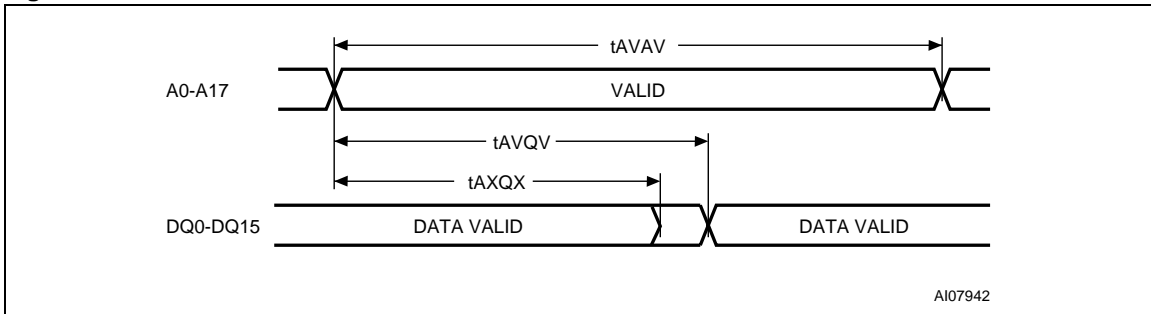
Figure 17. SRAM Read Mode AC Waveforms, Address Controlled
