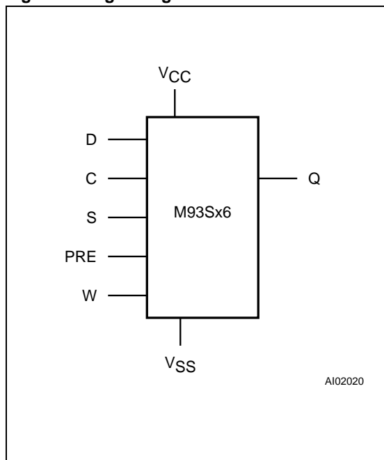
Figure 2. Logic Diagram
