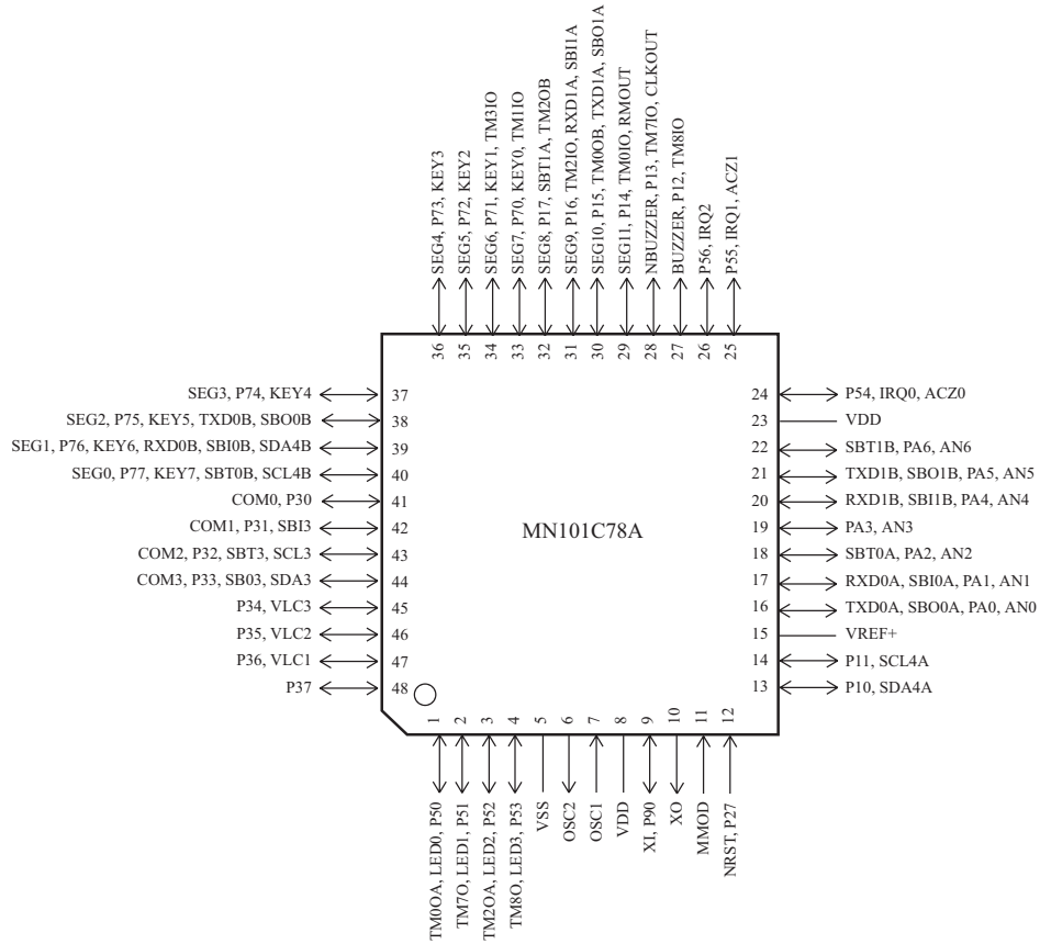
TQFP048-P-0707B
