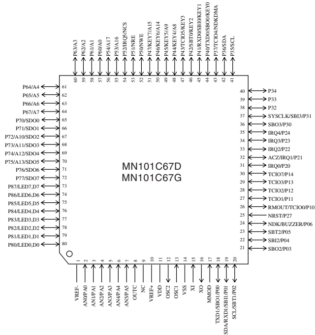
TQFP080-P-1212D *Lead-free
