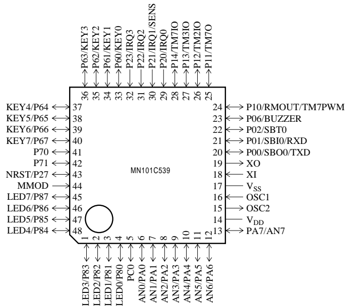
TQFP048-P-0707B *Lead-free
