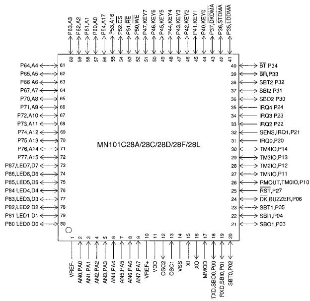
LQFP080-P-1414A (MN101C28A / 28C / 28D / 28F / 28L) TQFP080-P-1212 (MN101C28A / 28C / 28D)
