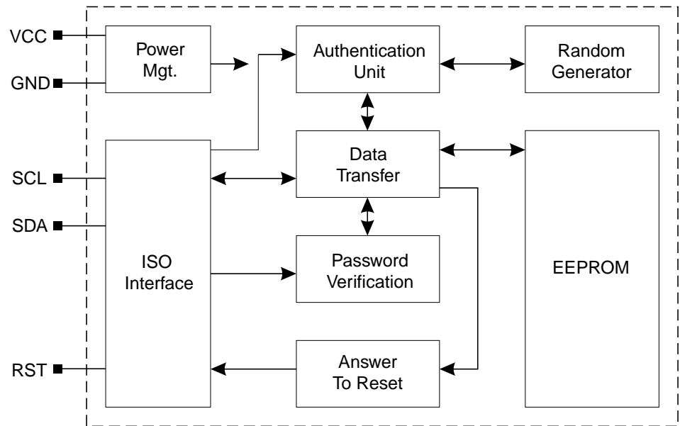
Figure 3. Block Diagram
