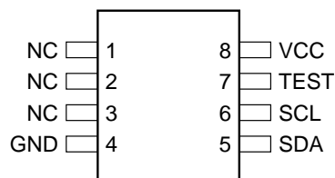
8-Pin SOIC
