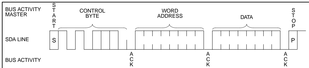
FIGURE 5-1: BYTE WRITE
