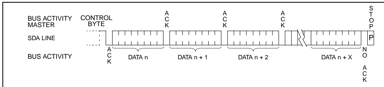
FIGURE 7-2: SEQUENTIAL READ
