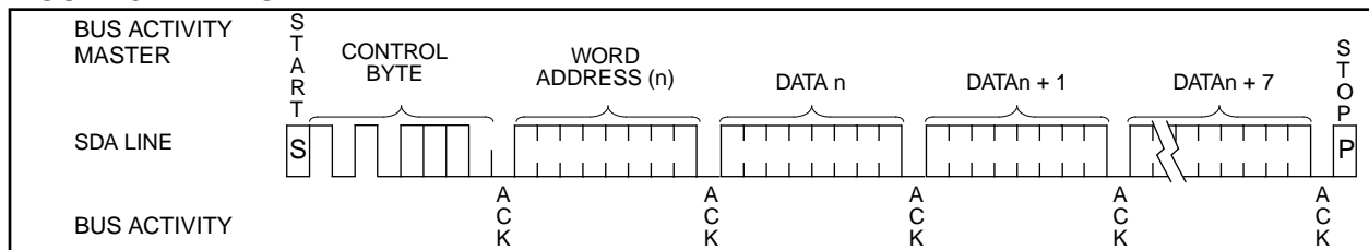
FIGURE 5-2: PAGE WRITE
