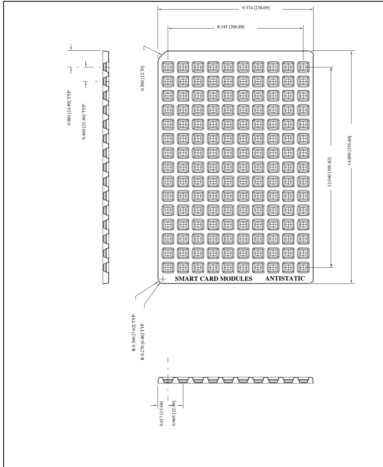
FIGURE 8-1: TRAY DIMENSIONS
