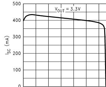
Short Circuit Current vs Output Voltage
