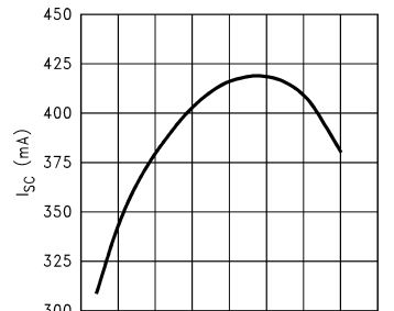
Instantaneous Short Circuit Current vs Temperature
